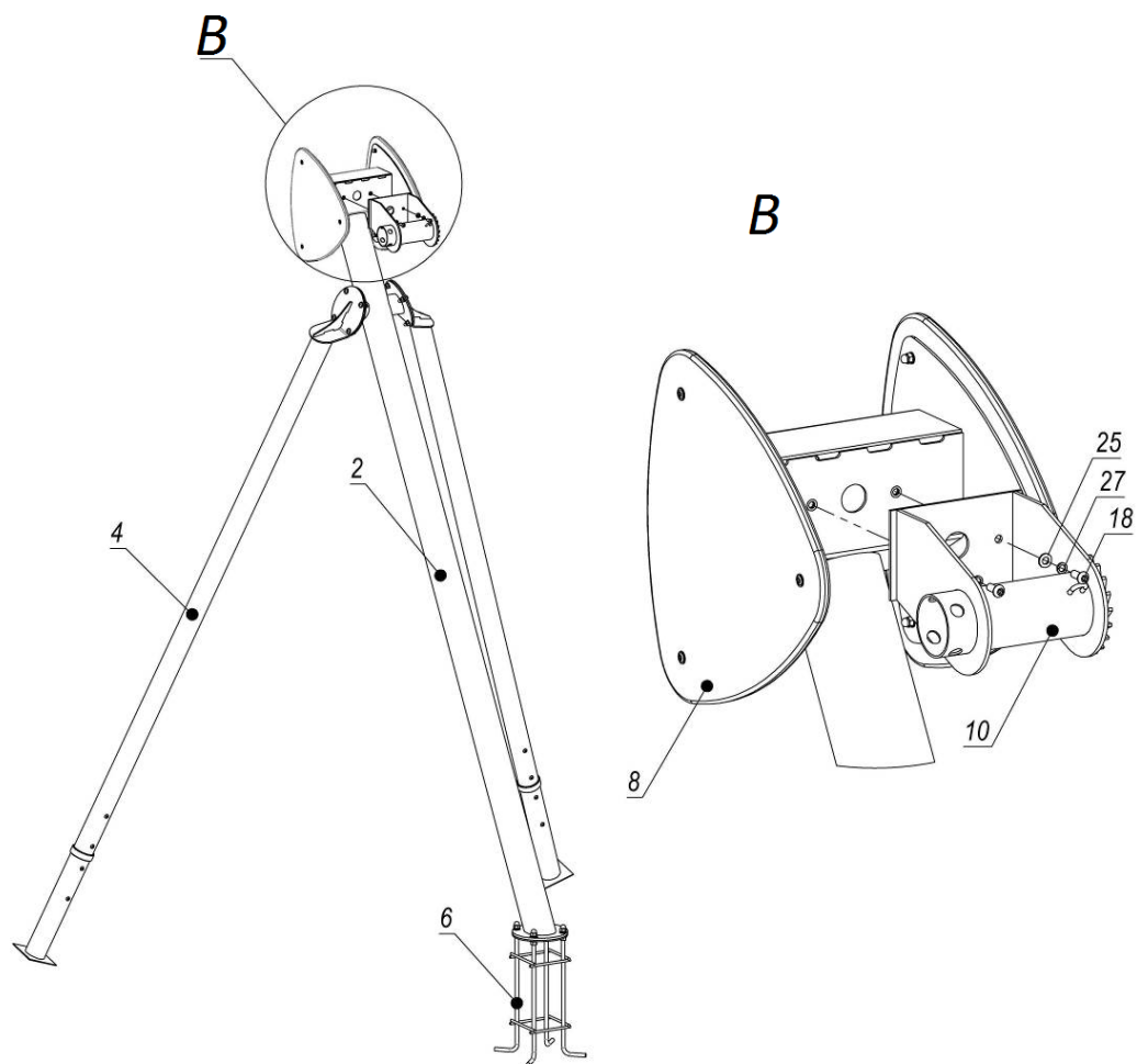
Picture 3 – Installation scheme of tensioning device
