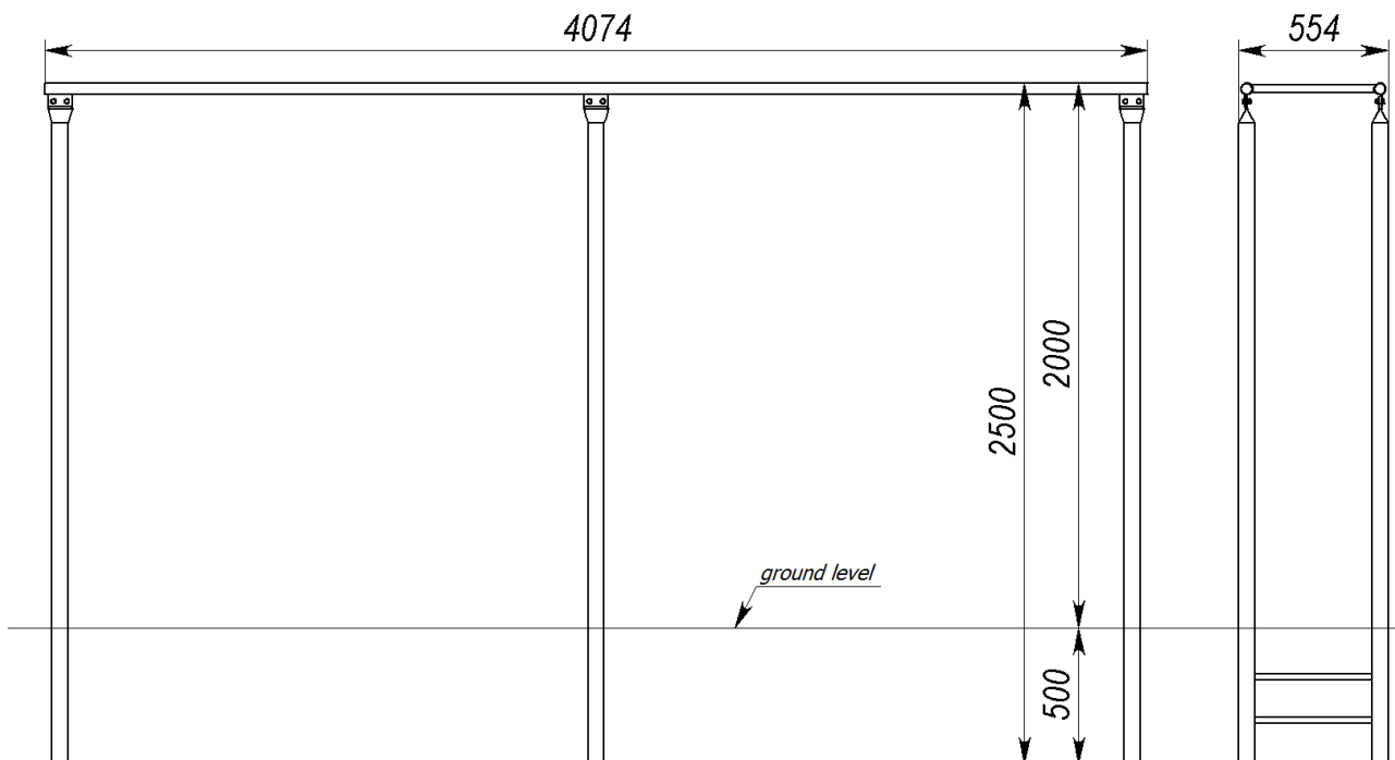
Pic. 2 Overall dimensions
