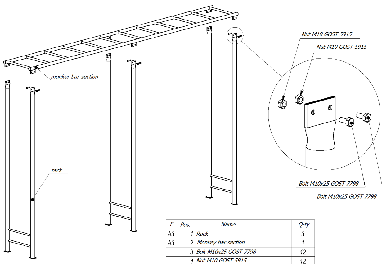
Pic. 1 Components and assembly procedure
