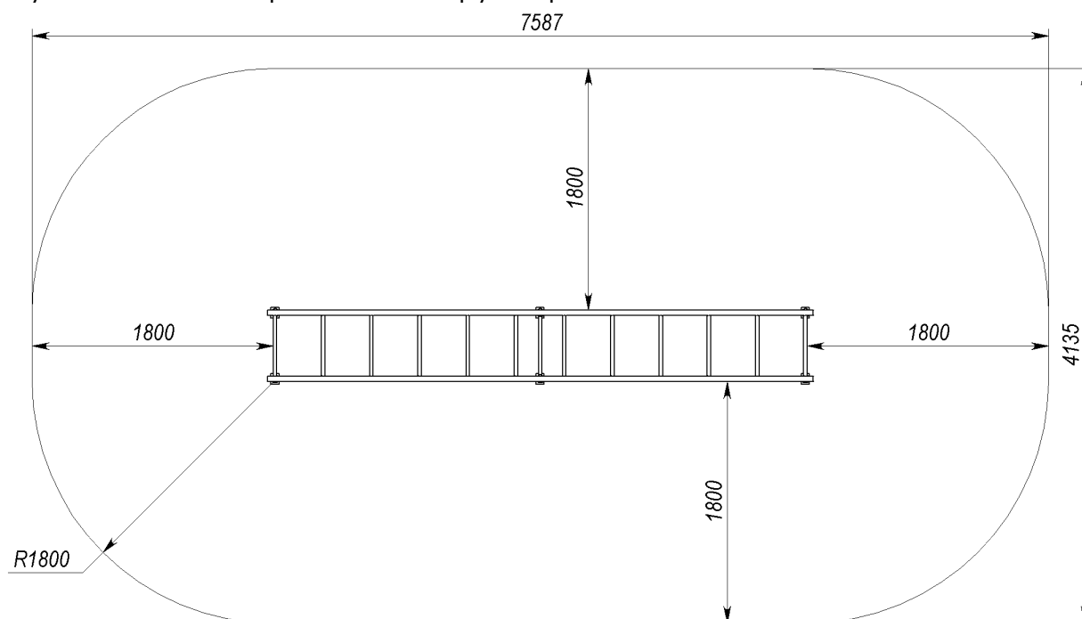
Pic. 4 Safety zone
