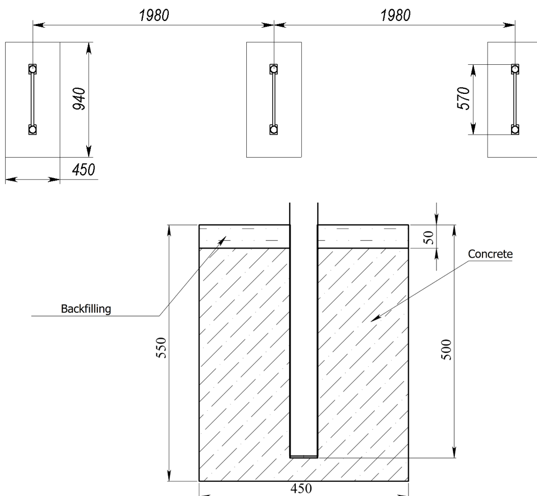
Pic. 3 Scheme of foundation installation
