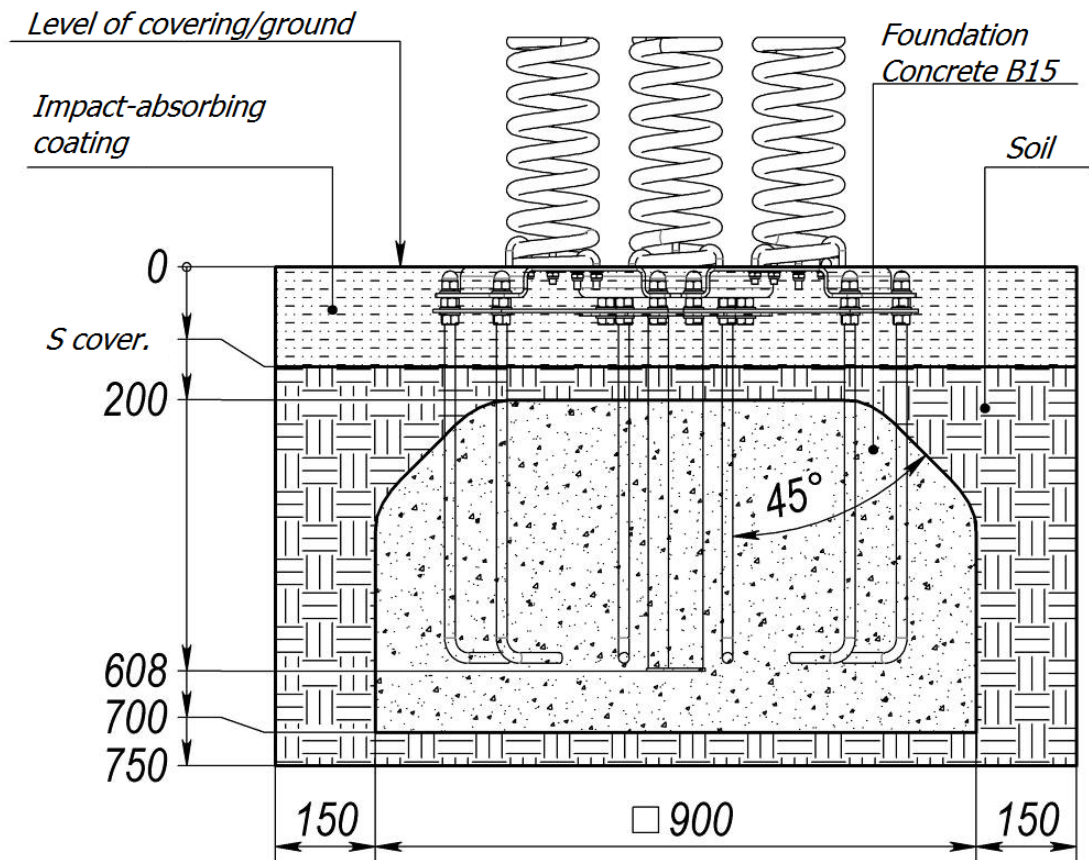
Picture 3 - Concreting scheme of the central embedded element
