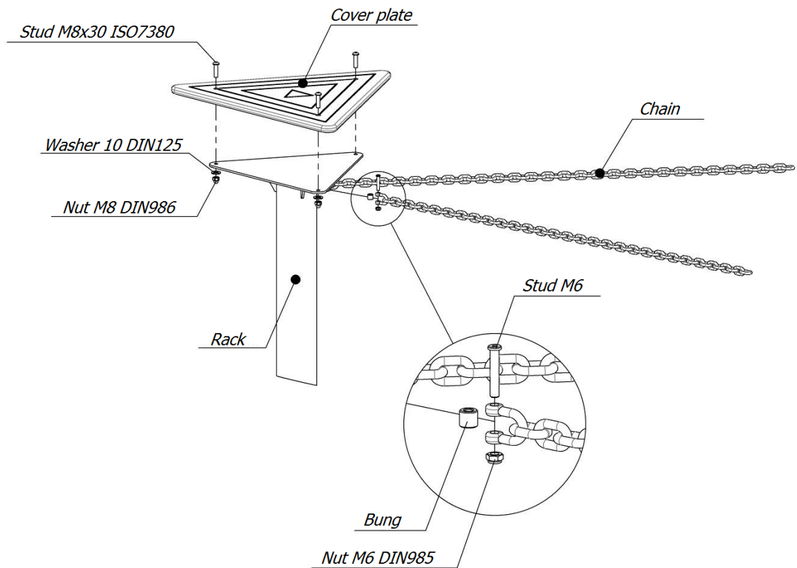
Picture 2 – Fastening scheme for cover plates and chains
