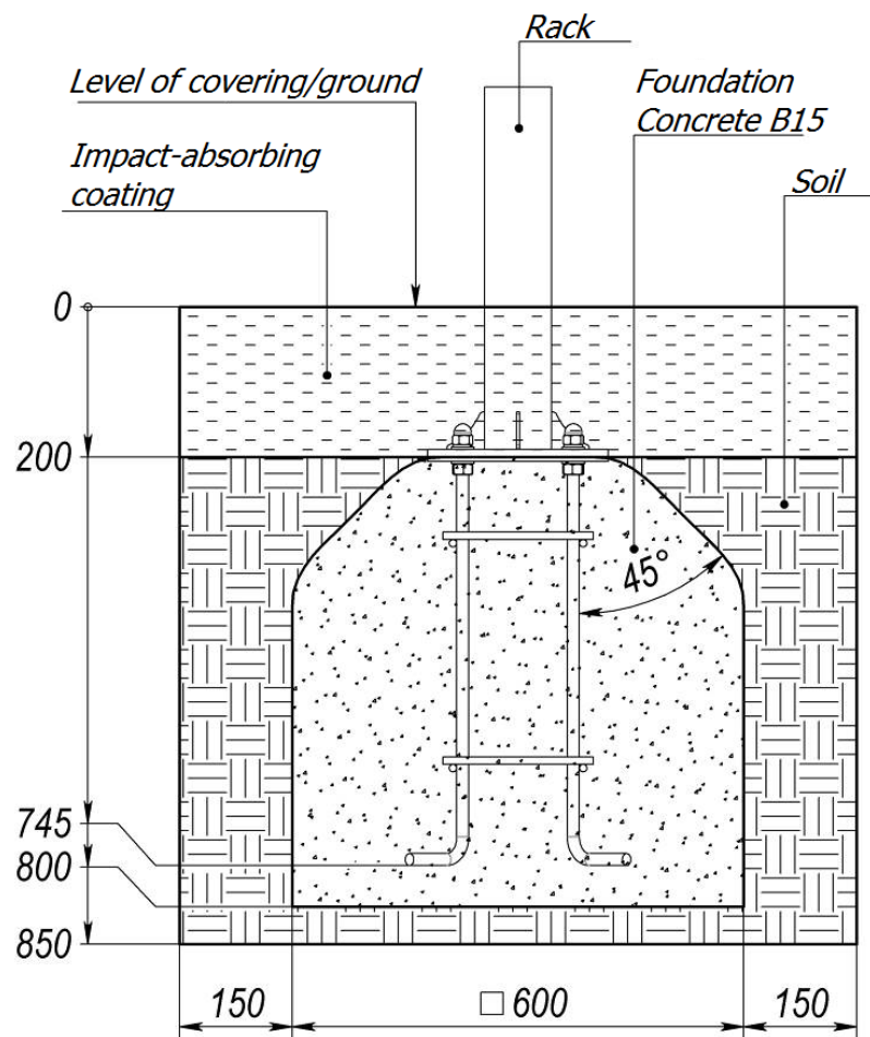
Picture 4 – Concreting scheme of embedded element (Pos. №5 in Appendix)
