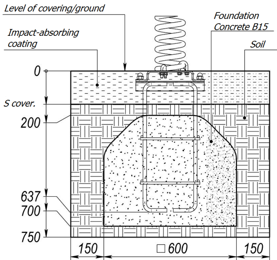
Picture 5 – Concreting scheme of embedded element (Pos. №3 in Appendix)
