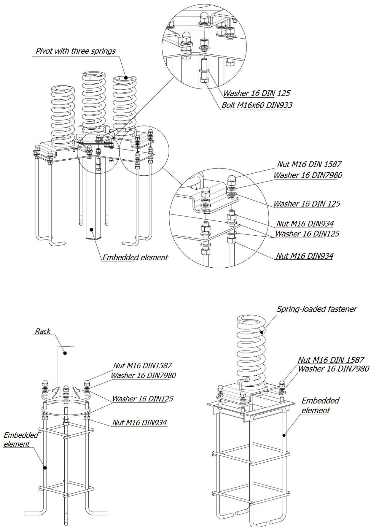
Picture 1 – Assembling scheme of embedded elements
