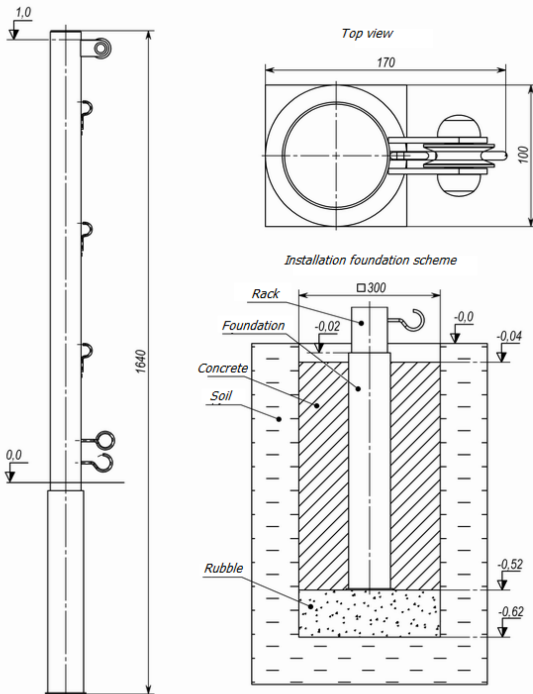
Picture 2 «Product overall dimensions and installation scheme»
