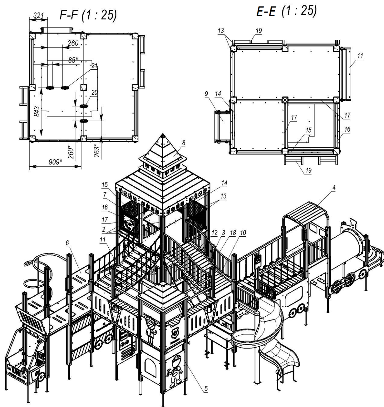
Picture 4- Overall dimensions of the complex
