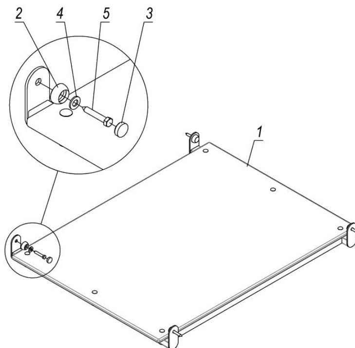
Picture 22 – Assembly scheme of straight railings
