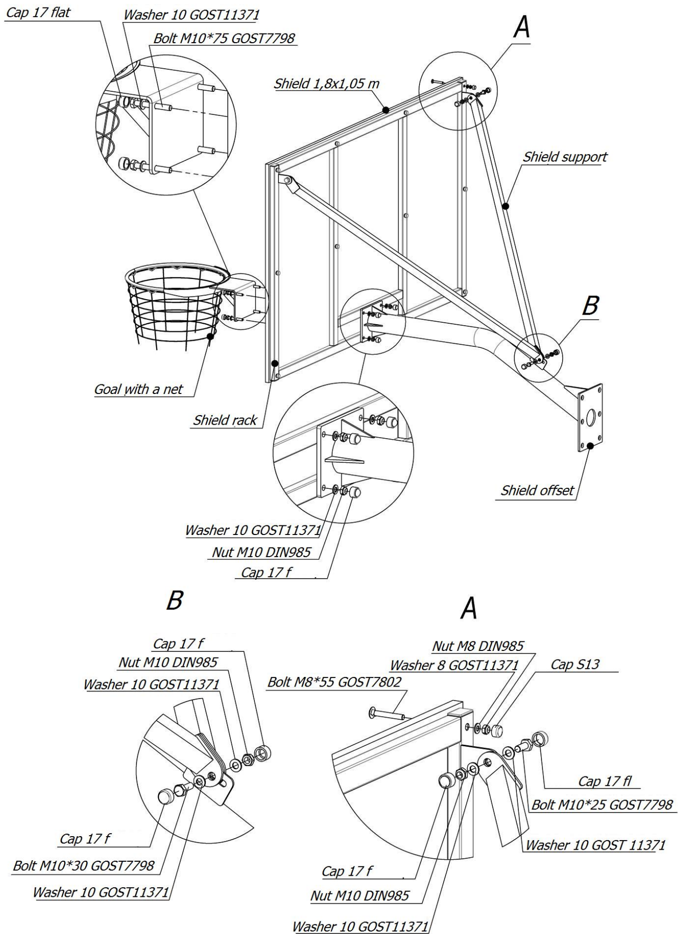
Picture 2 – Assembly scheme 1
