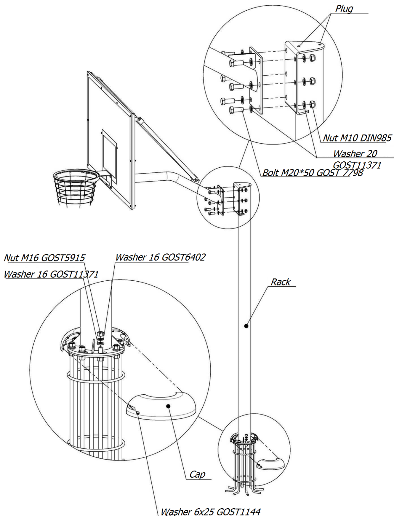
Picture 4 – Installation scheme 3
