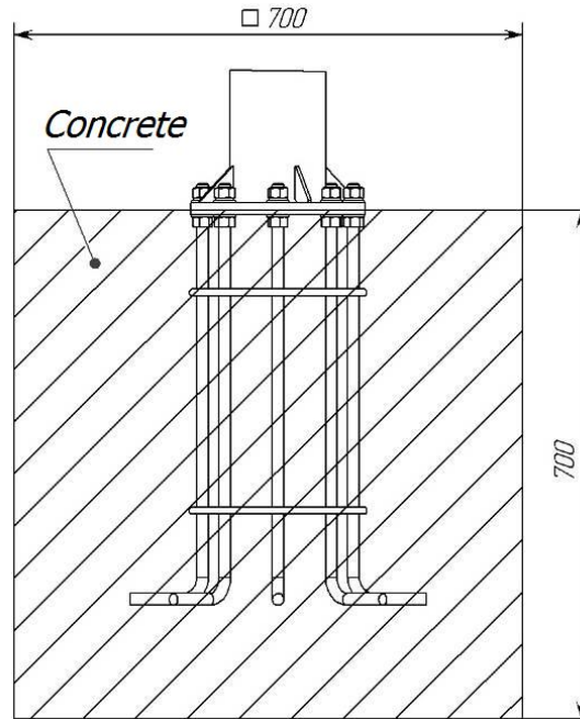
Picture 5 – Concreting scheme
