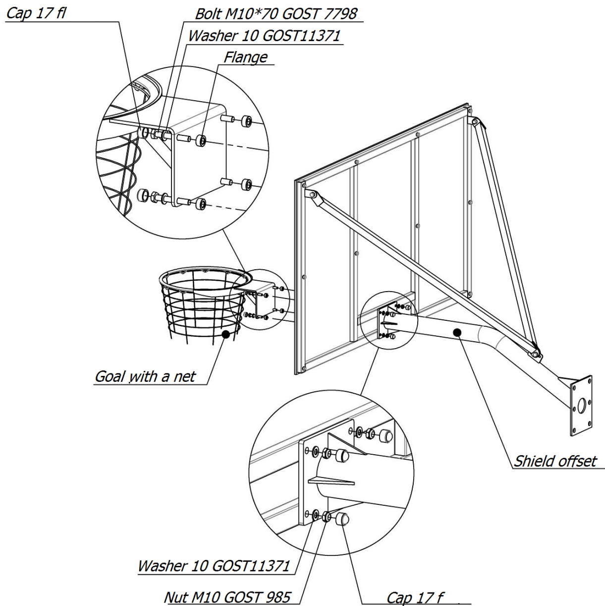
Picture 3 – Basketball goal fixing scheme for UT410.1
