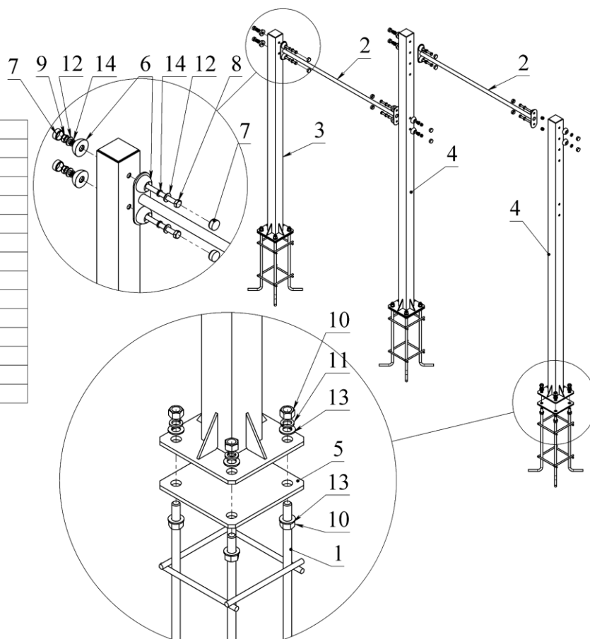
Picture 2. Assembly scheme
