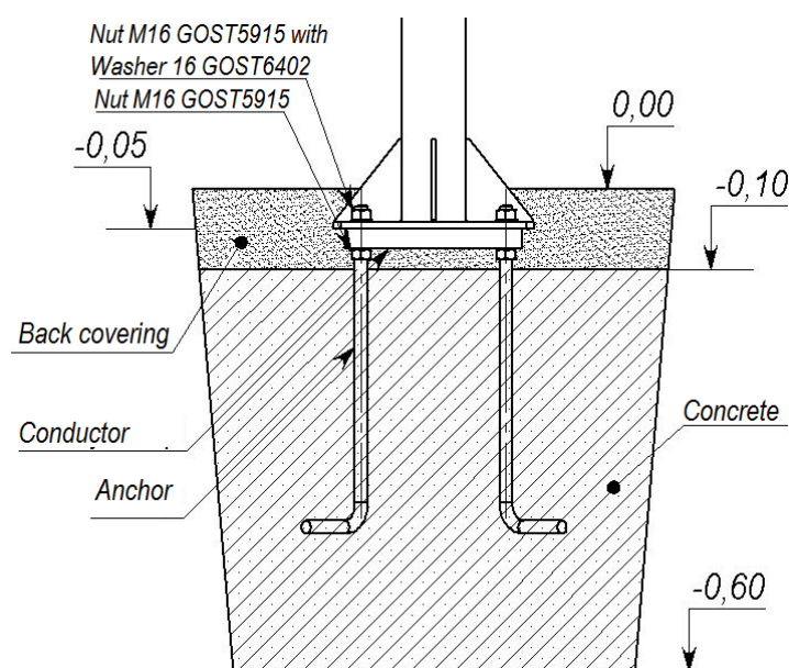
Picture 1. Foundations assembly scheme
