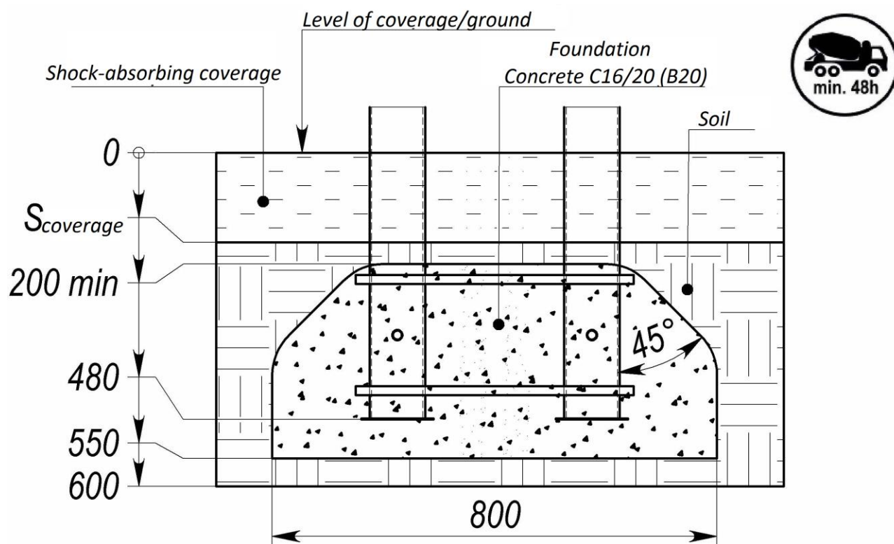
Picture 1 – Concreting scheme
