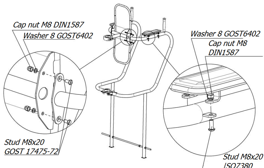
Picture 3 - Installation scheme for the abs support
