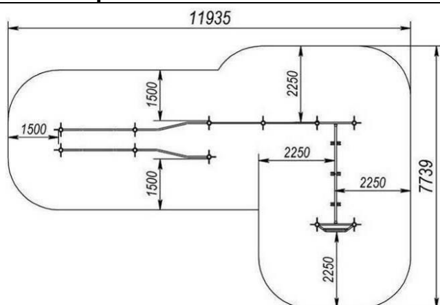
Installation variant №1
