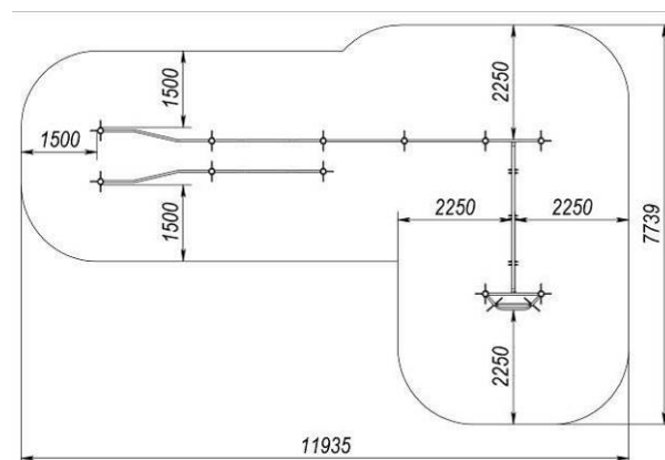
Installation variant №2
