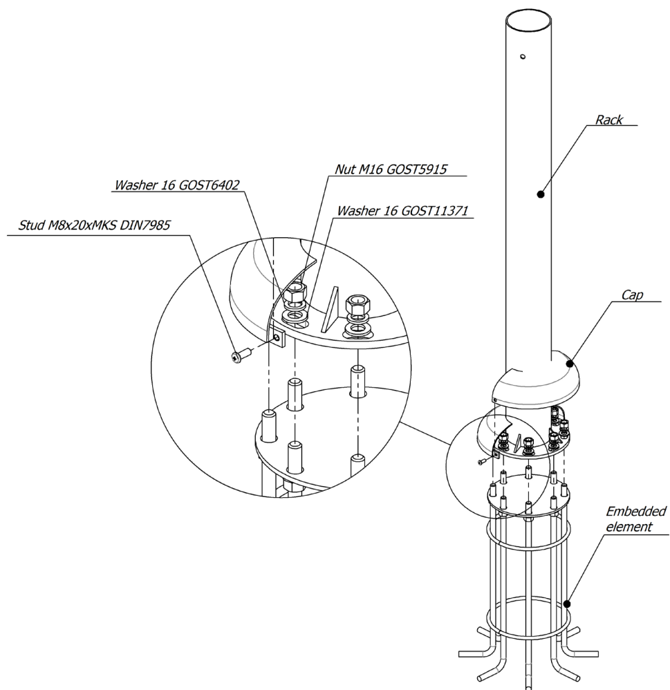
Picture 1 – Connection scheme of the rack with the embedded element
