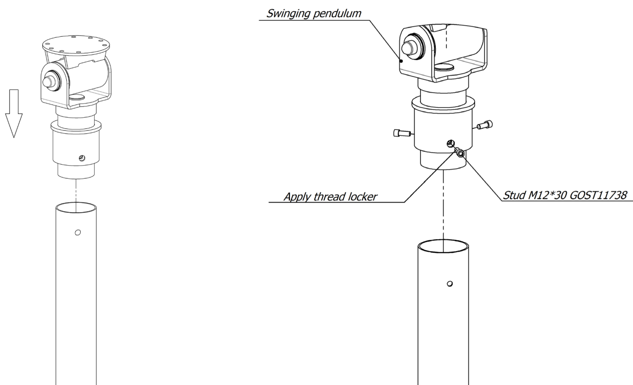
Picture 2 – Installation of the swinging pendulum
