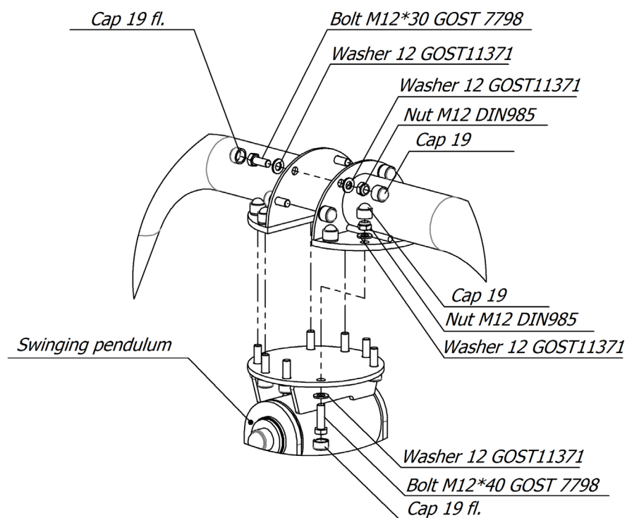
Picture 3 – Fasten the levers with the swing pendulum
