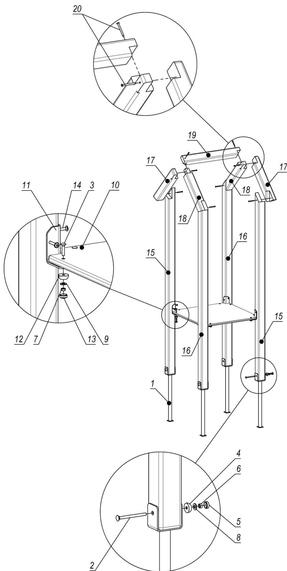
Picture 3 – Tower assembly scheme
