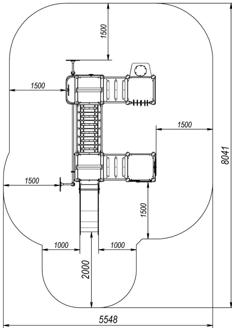
Picture 1 - Installation area and landing zone
