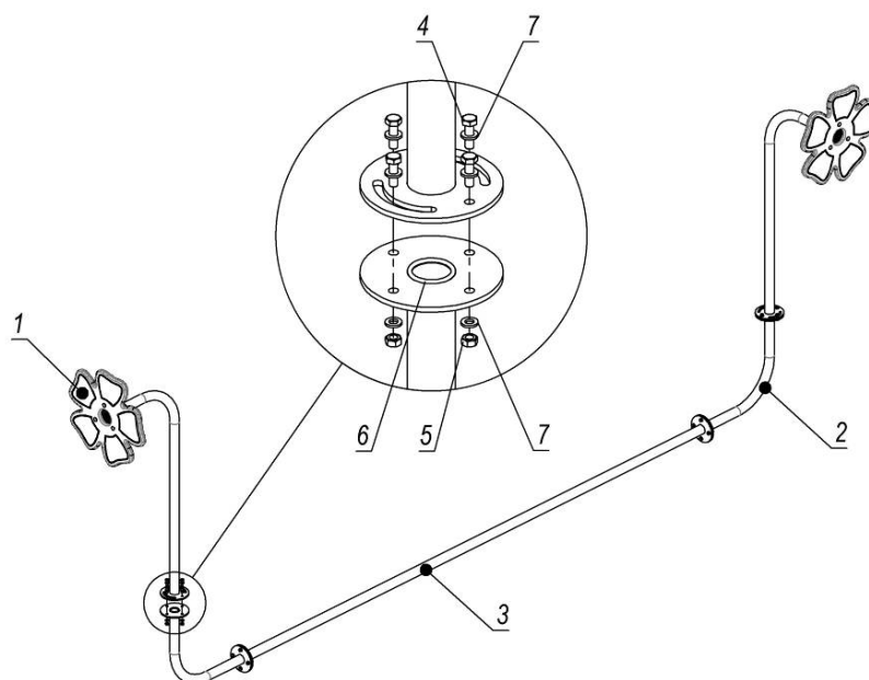
Picture 7 – Panel assembly scheme (assembly of other panels is identical)
