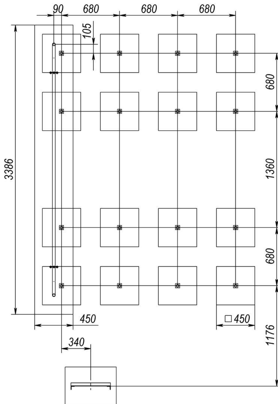
Picture 2 – Layout scheme of foundations
