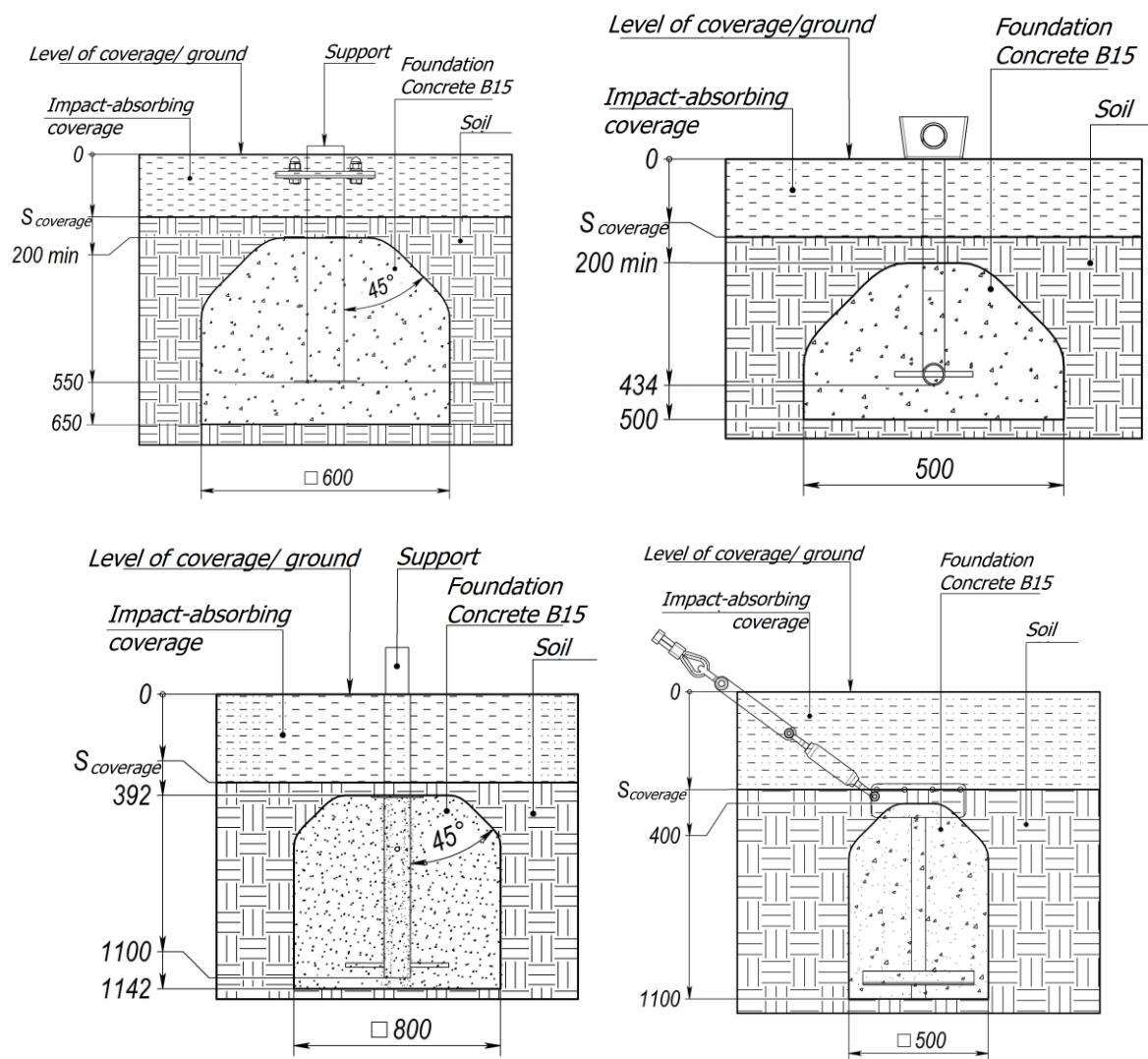
Picture 1 – Concreting schemes (Concrete placement scheme in concreting zone)
