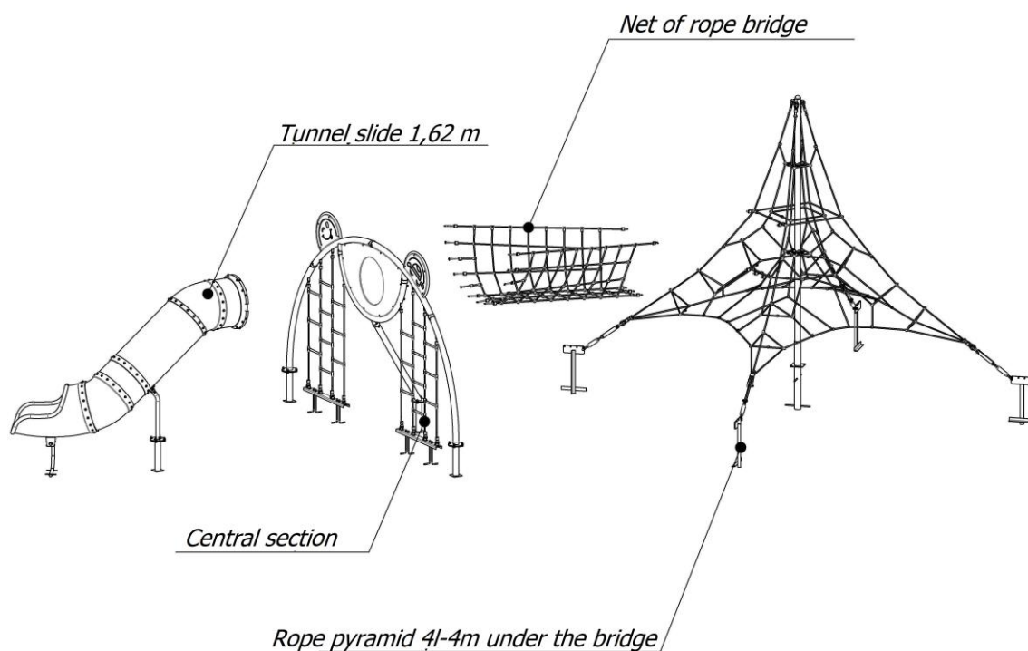
Picture 2 – Scheme of complex parts installation
