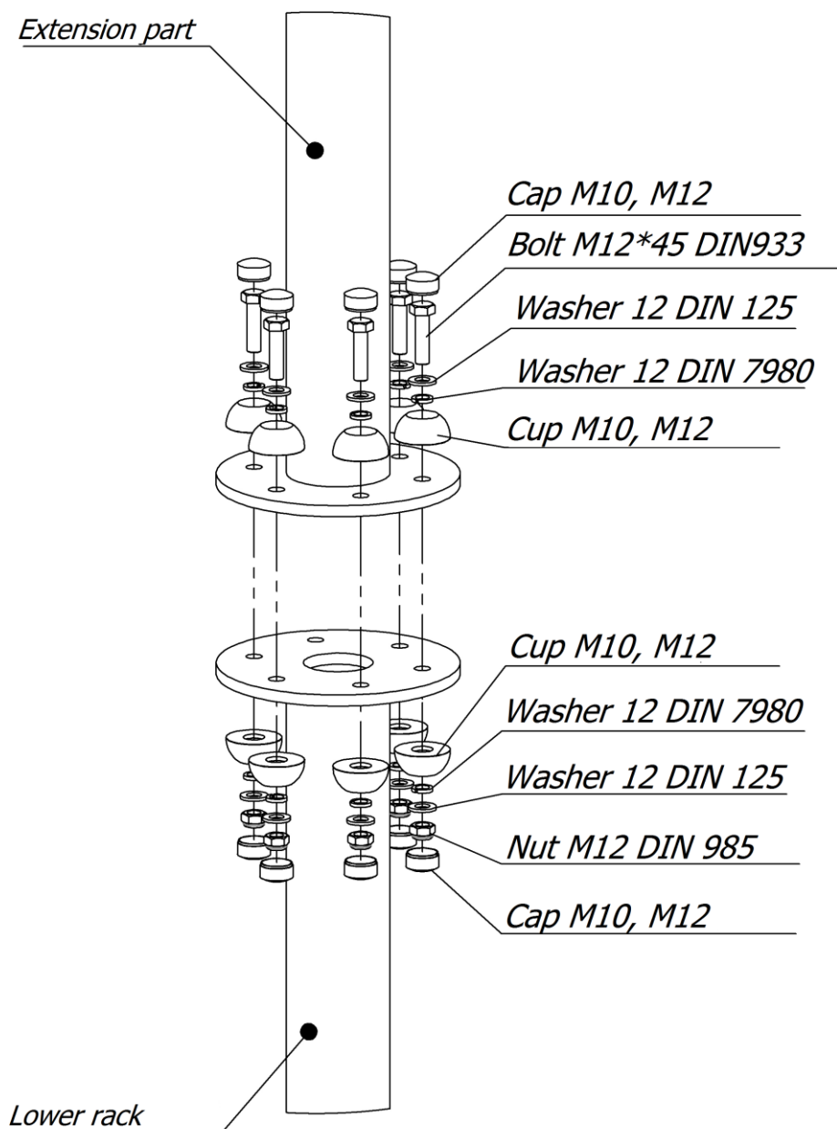
Picture 9 – Fix rope pyramid between extension cord and rack
