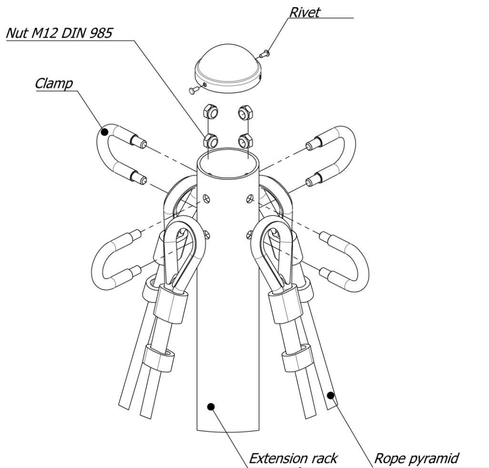
Picture 10 – Fix the rope with clamps
