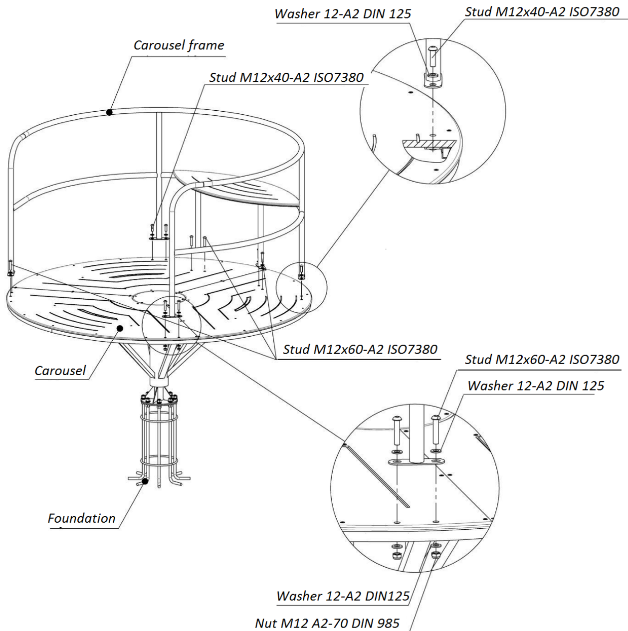
Picture 1 – Carousel framework assembly scheme LK484, LK484.1
