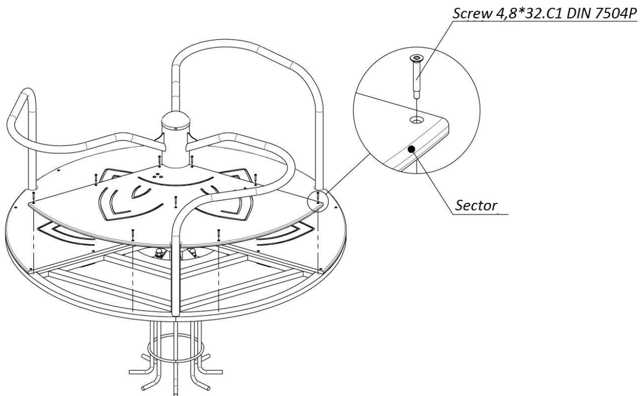
Picture 4 – Sector for LK481, LK481-S, LK481.1, LK481.1-S, LK483, LK483.1, LK485, LK485.1, LK486, LK486.1, LK487, LK487.1 assembly scheme
