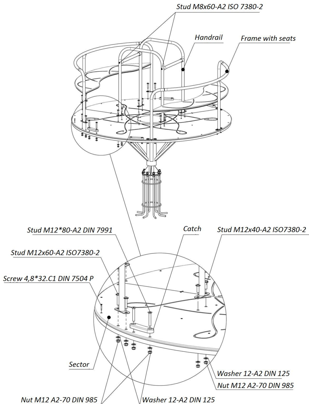
Picture 2 – Carousels LK488, LK488.1 assembly scheme
