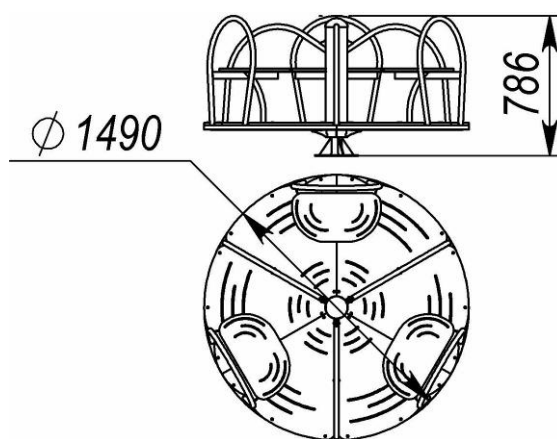
LK483, LK483.1 Carousel
