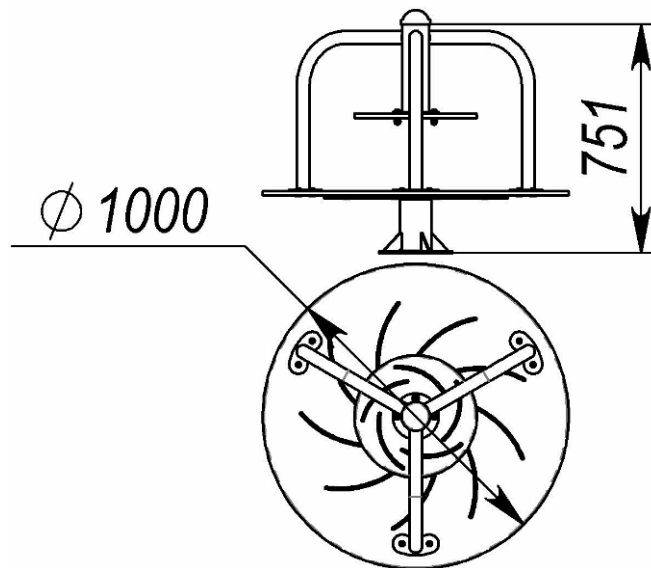
LK483, LK483.1 Carousel
