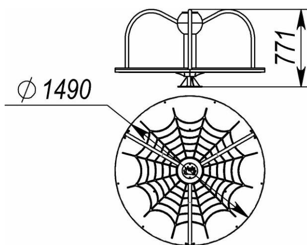
LK485, LK485.1 Carousel
