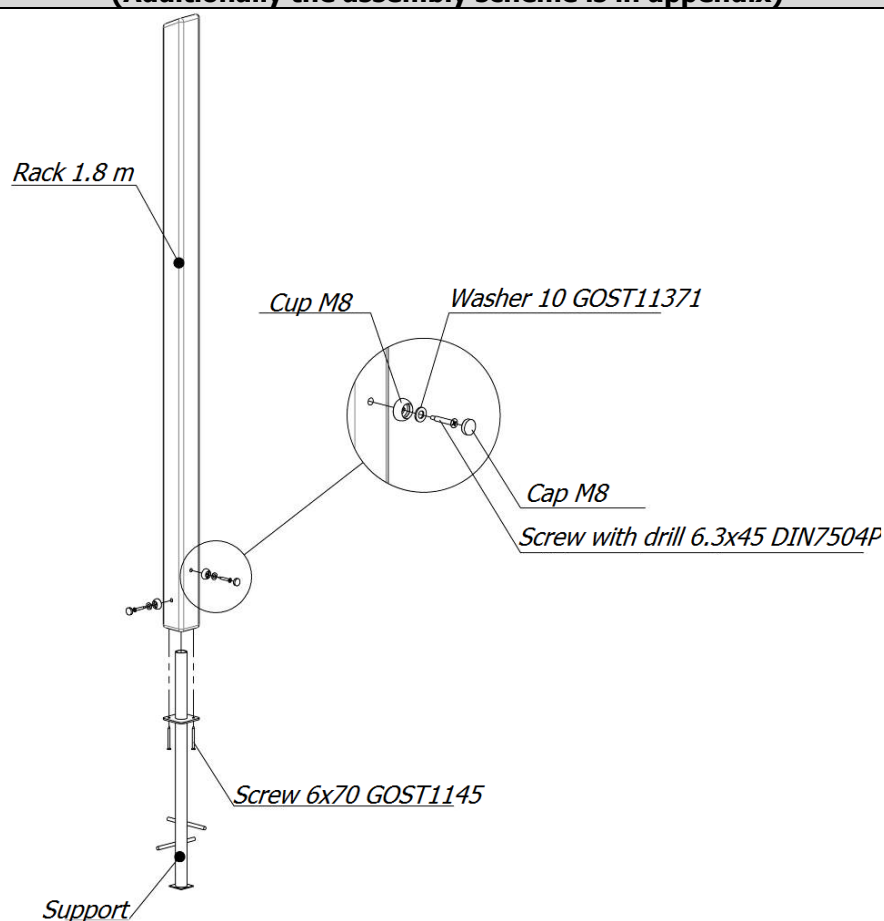
Picture 1 – Rack assembly scheme
