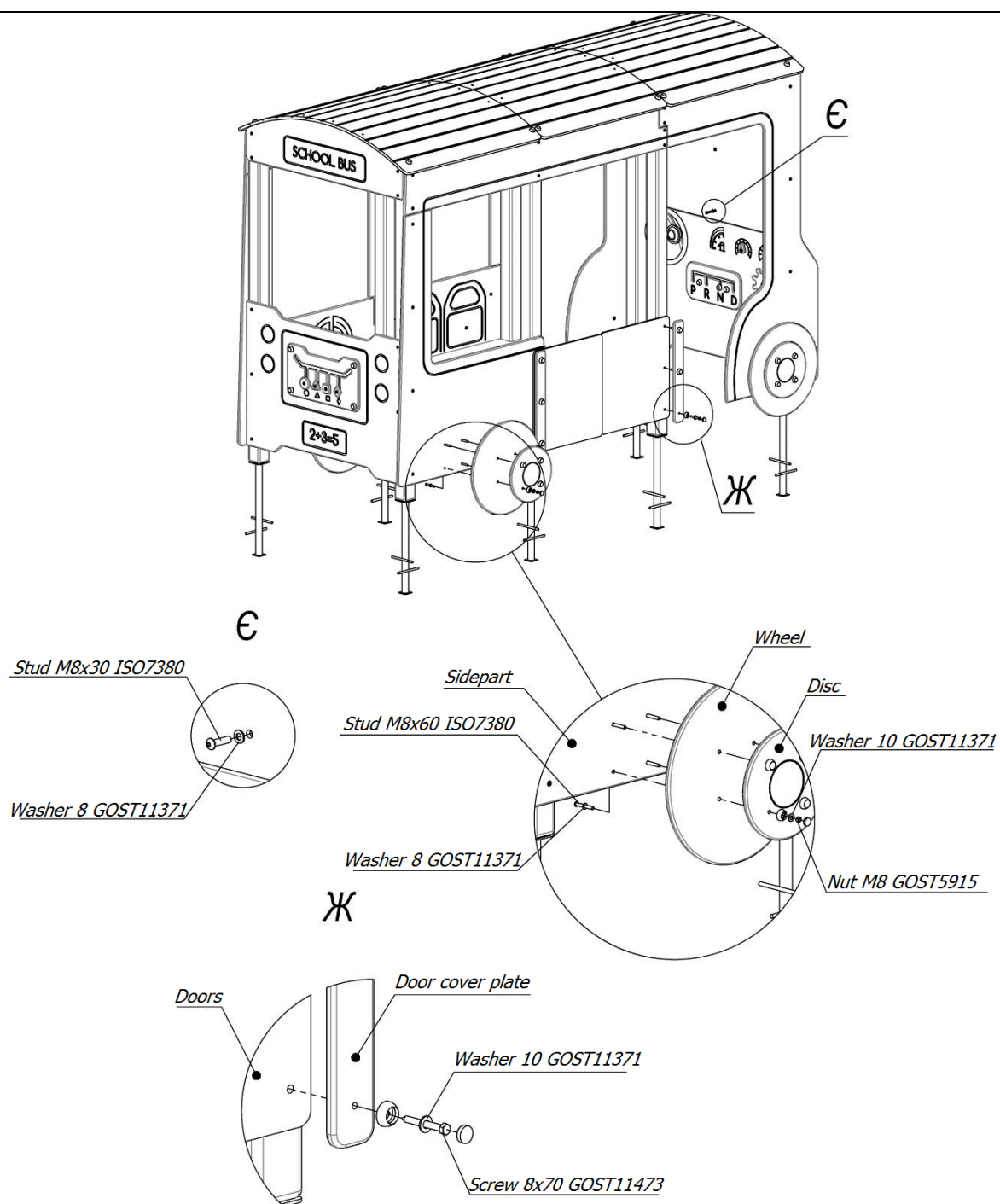
Picture 4 – Assembly scheme of wheels and cover plates
