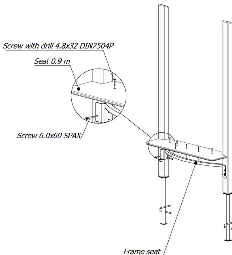
Picture 2 – Seat fastening scheme
