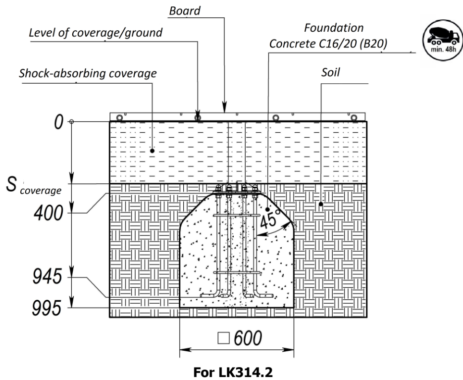
Picture 1 – Concreting scheme
