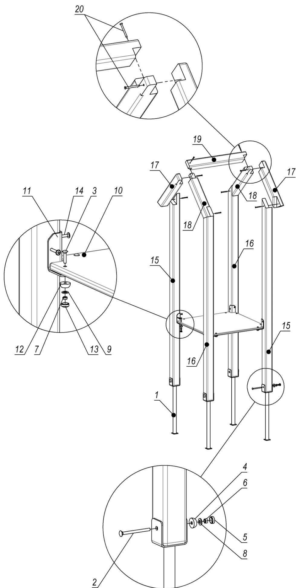
Picture 4 – Tower assembly scheme
