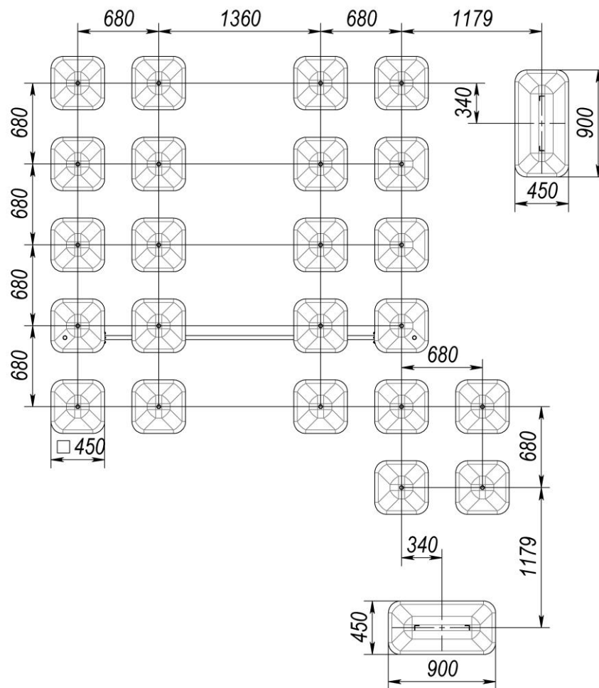
Picture 2 – Layout of foundations
