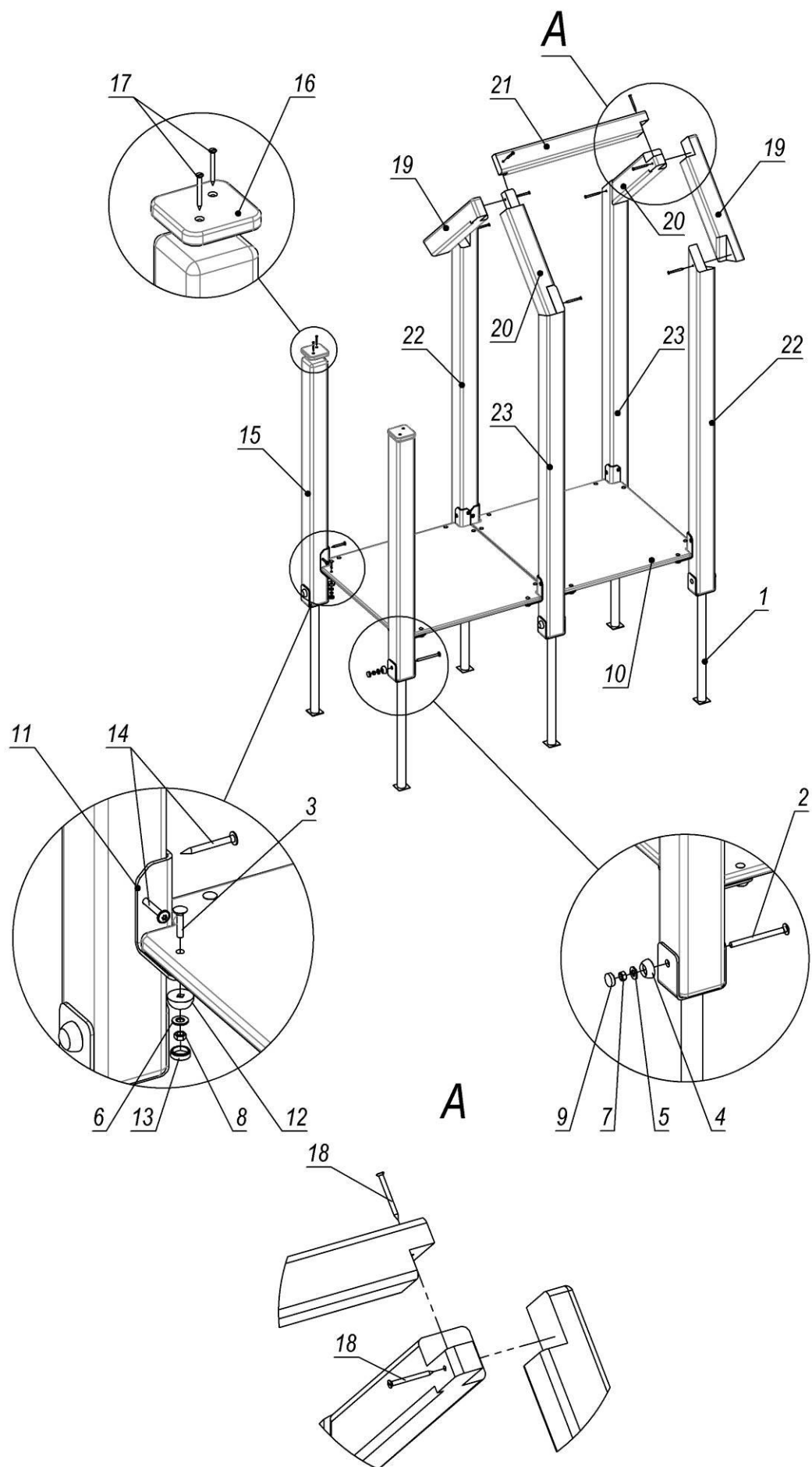
Picture 3 – House assembly scheme 0,76x1,44
