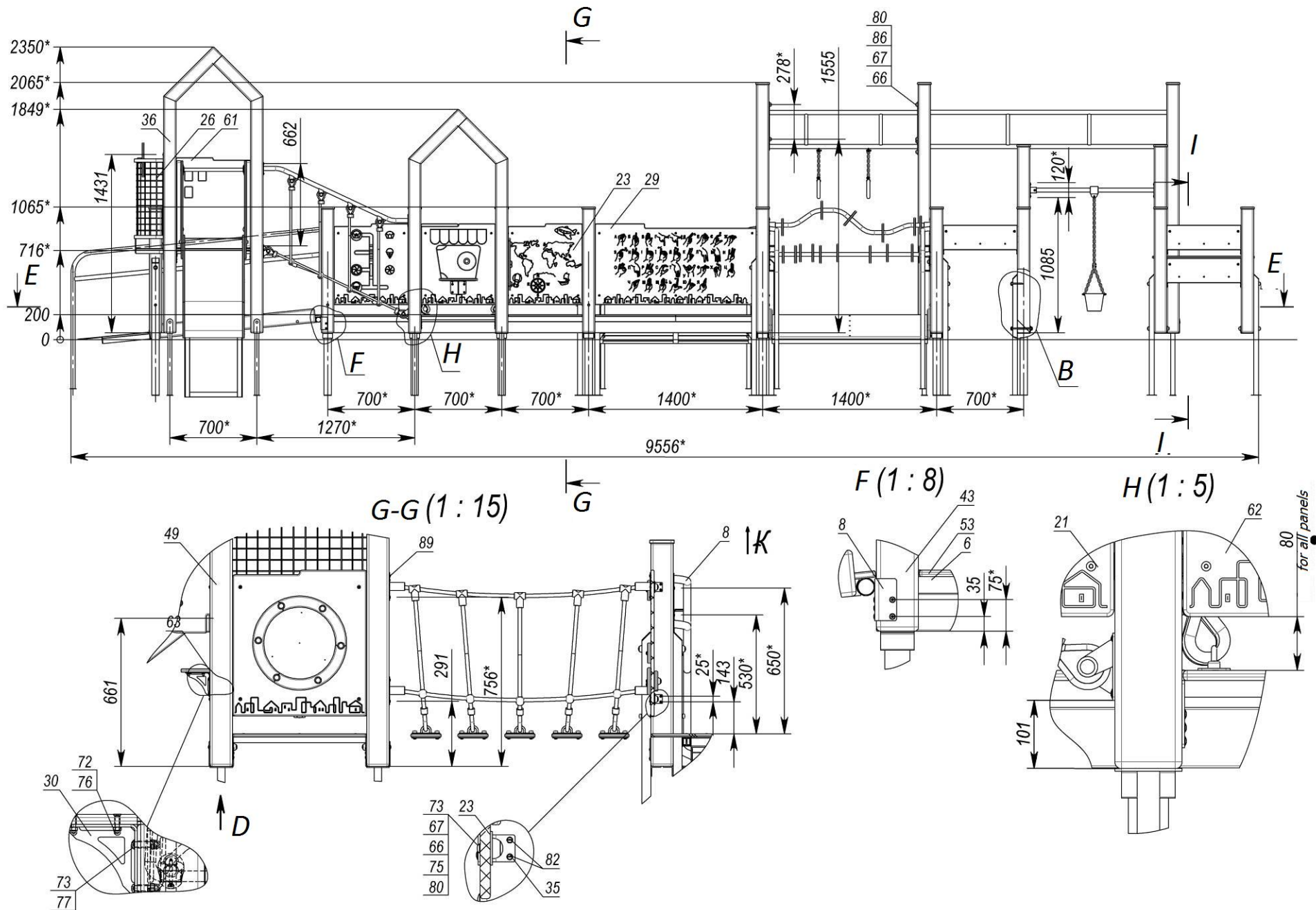
Picture 3 – Overall dimensions of the complex
