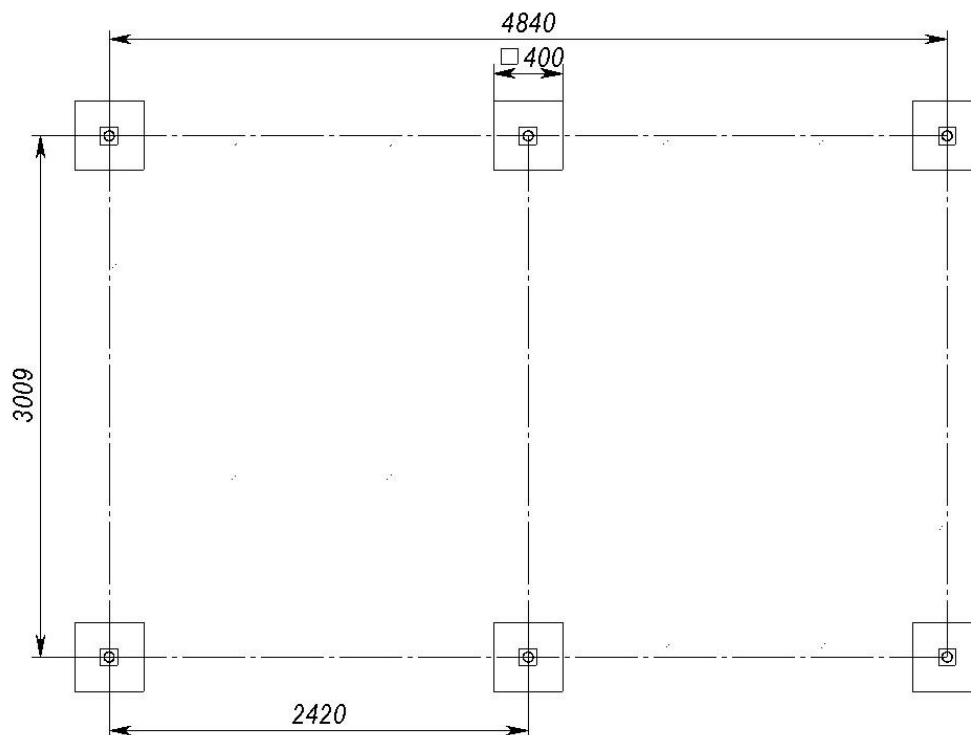
b) Marking the territory and the dimensions of the hole for UT502.1, UT502.1B
