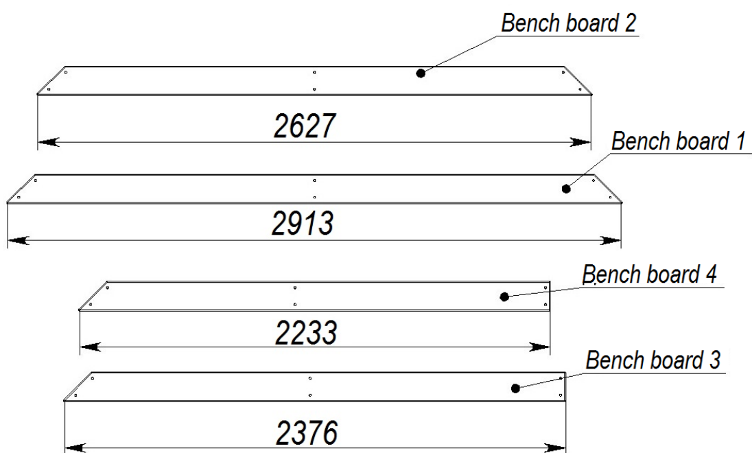
k) Boards overall dimensions
