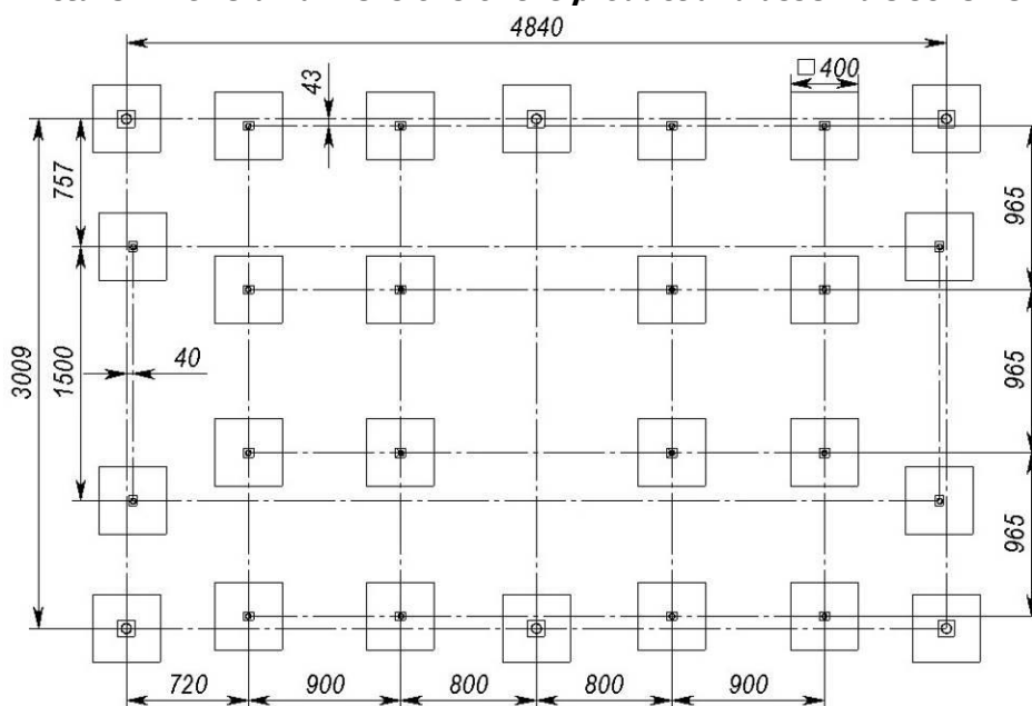
Picture 2 «Overall dimensions of the product and assemble scheme»
