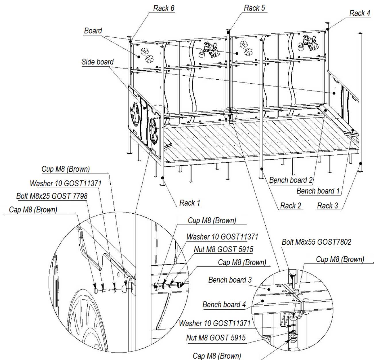
j) Side and back boards assembly scheme
