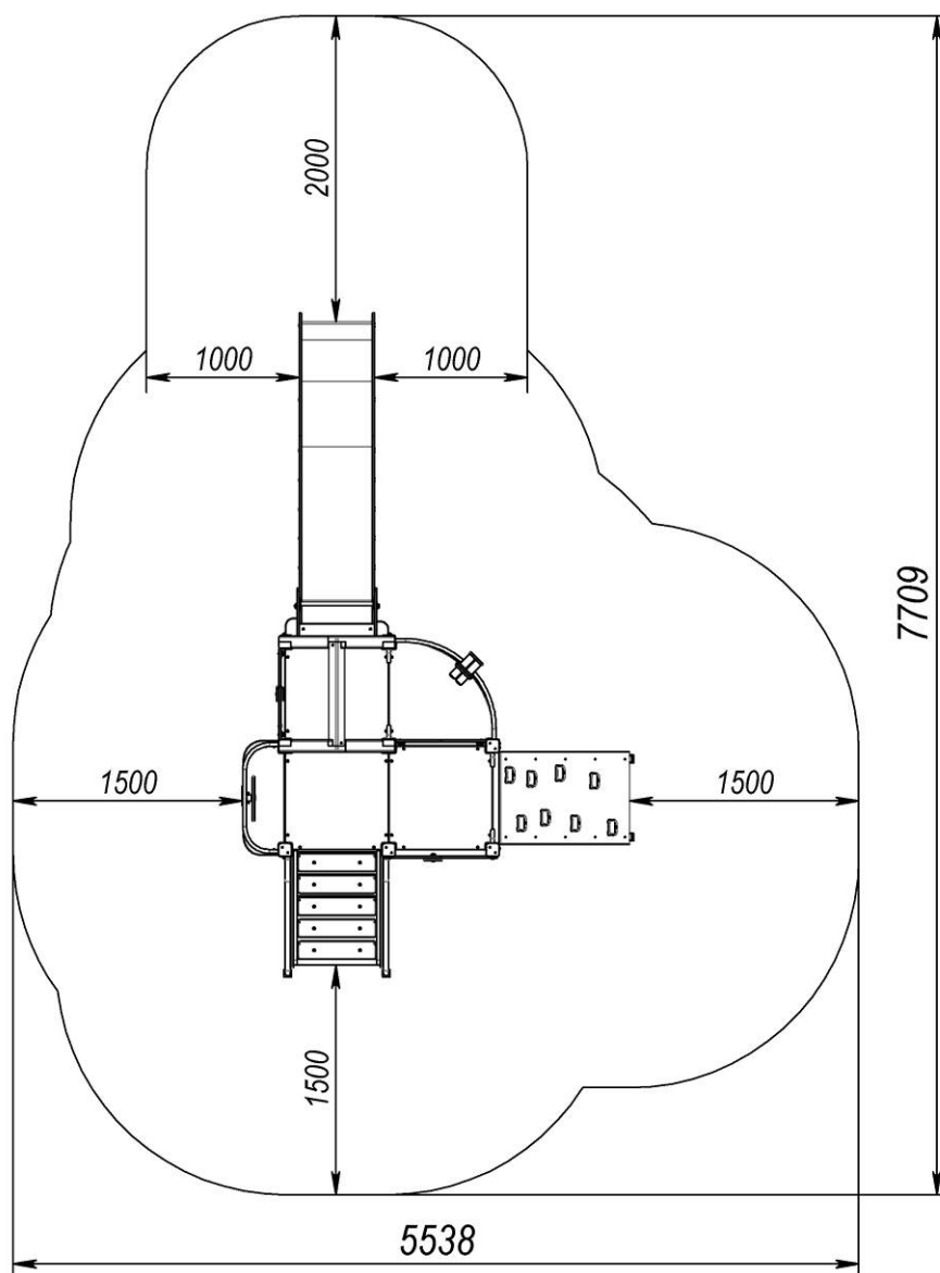
Picture 1 - Installation area and landing zone
