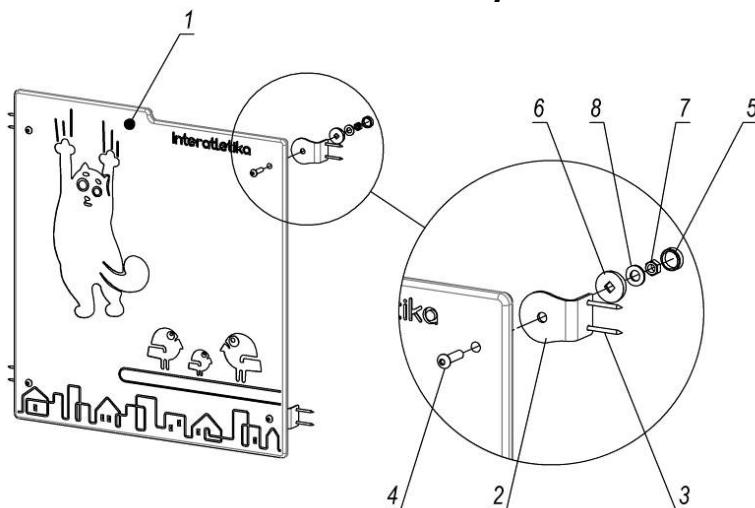
Picture 8 – Seat assembly scheme
