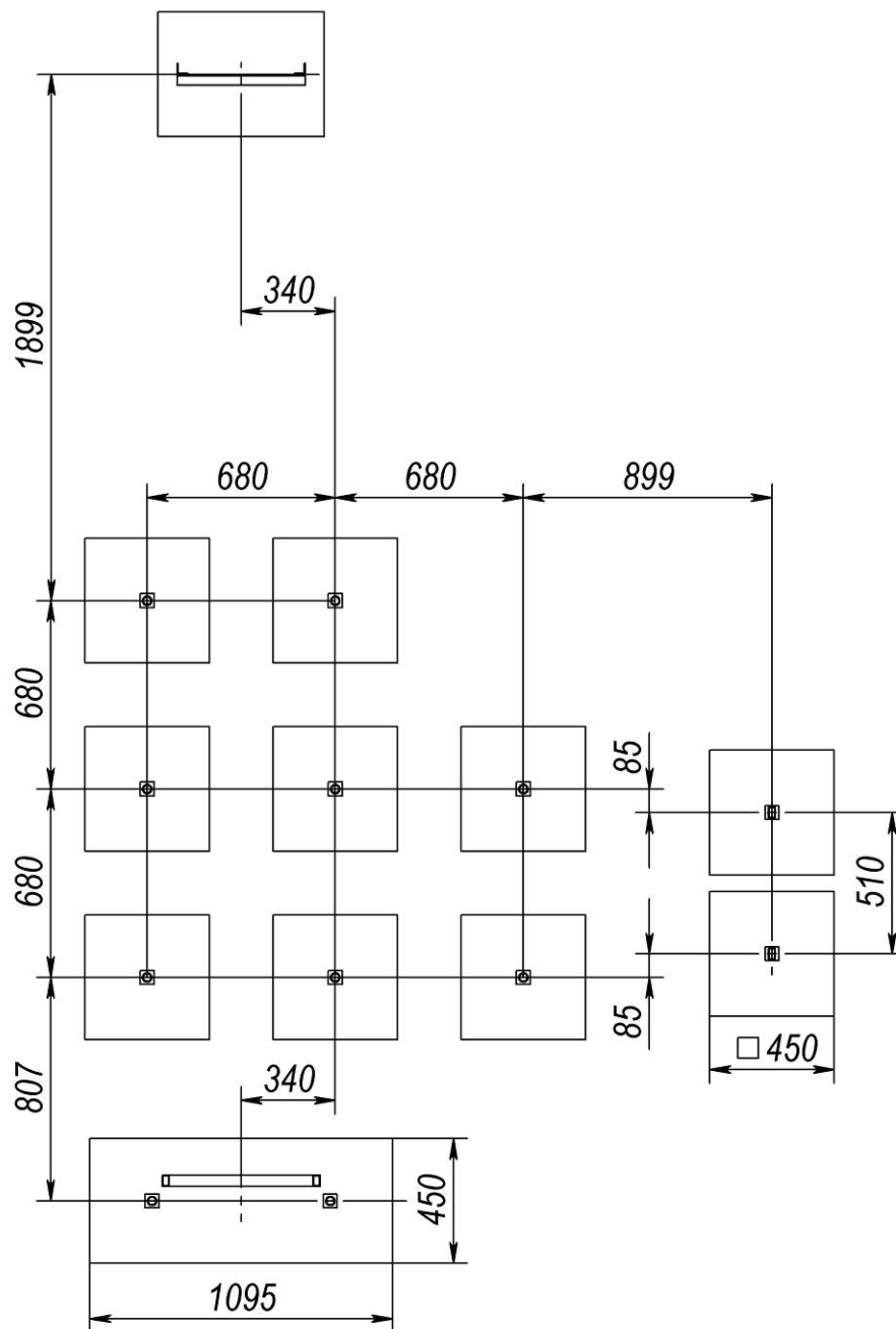
Picture 2 – Layout of the foundations
