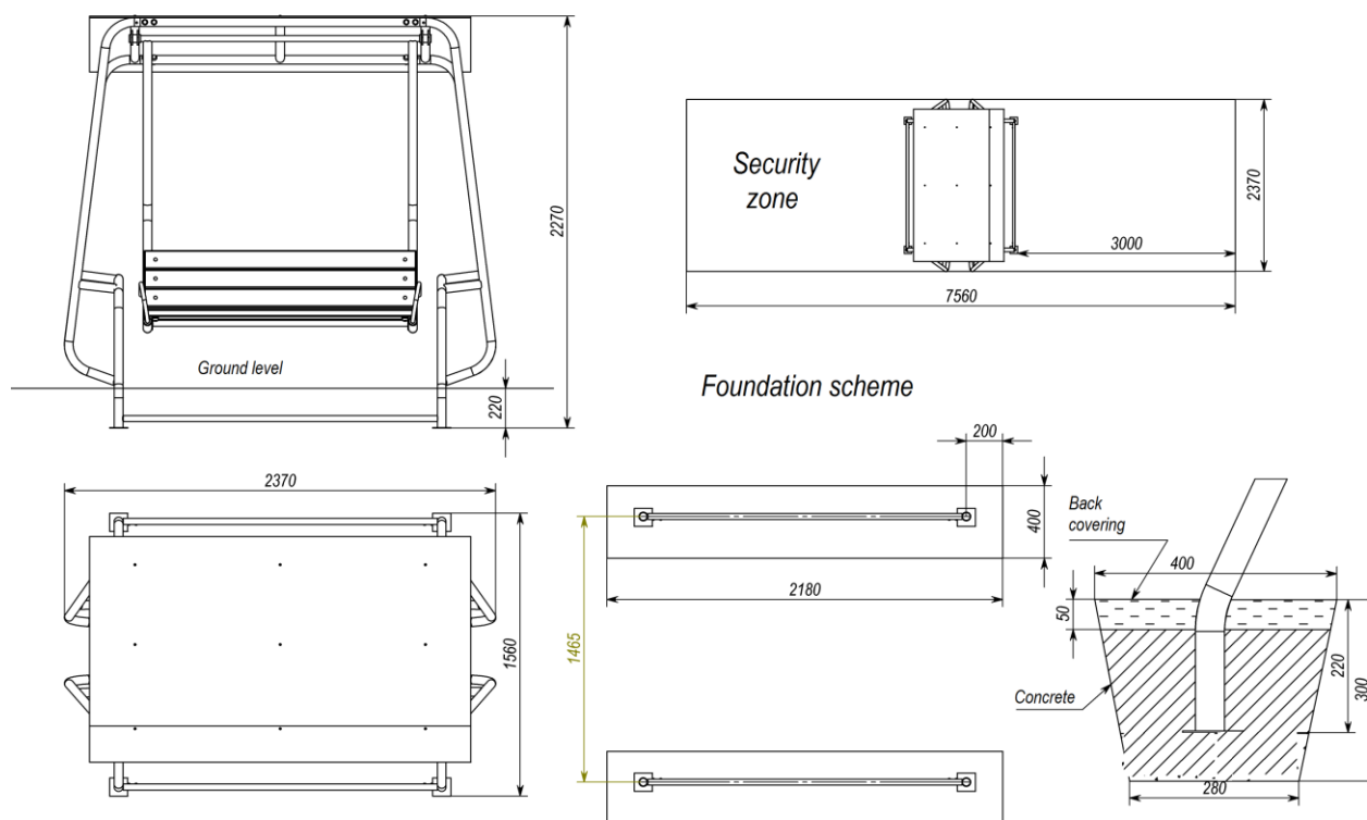
Picture 2. Foundation overall dimensions and installing scheme
