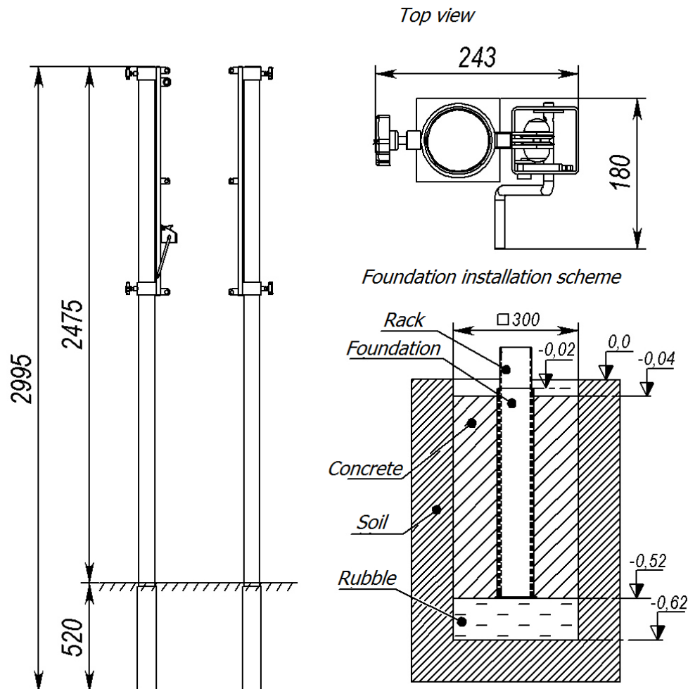
Picture 2 – Product overall dimensions and installation scheme
