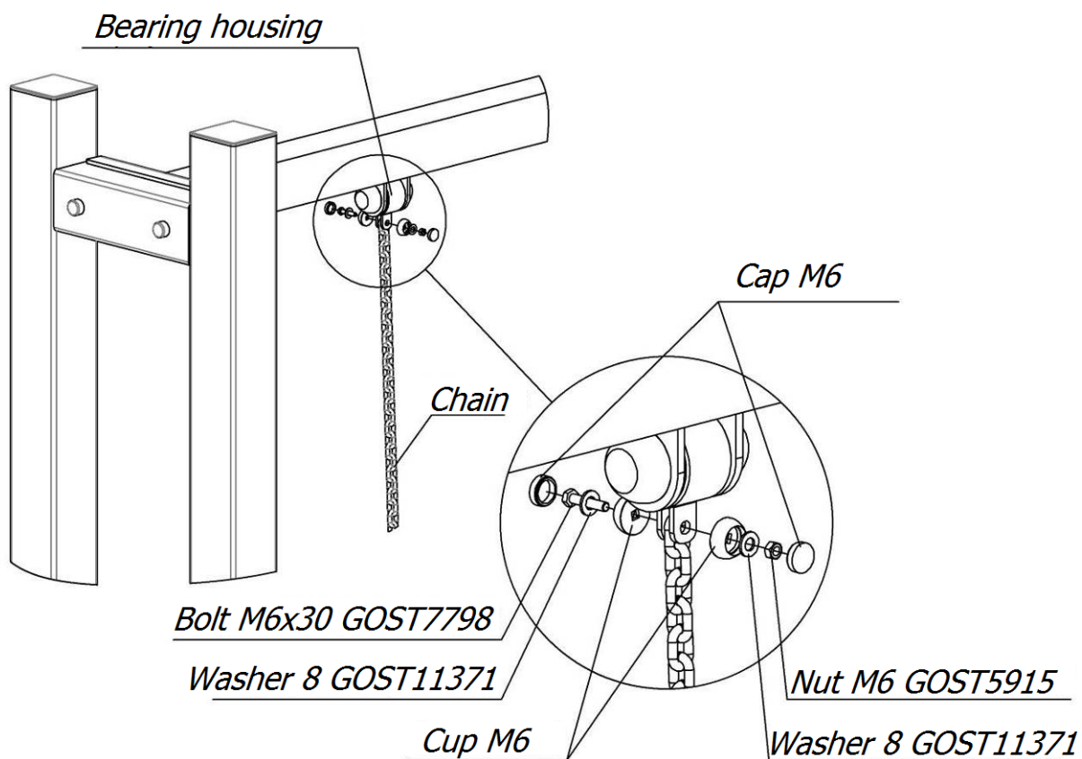
Picture 1 - Installation scheme of the crossbar
