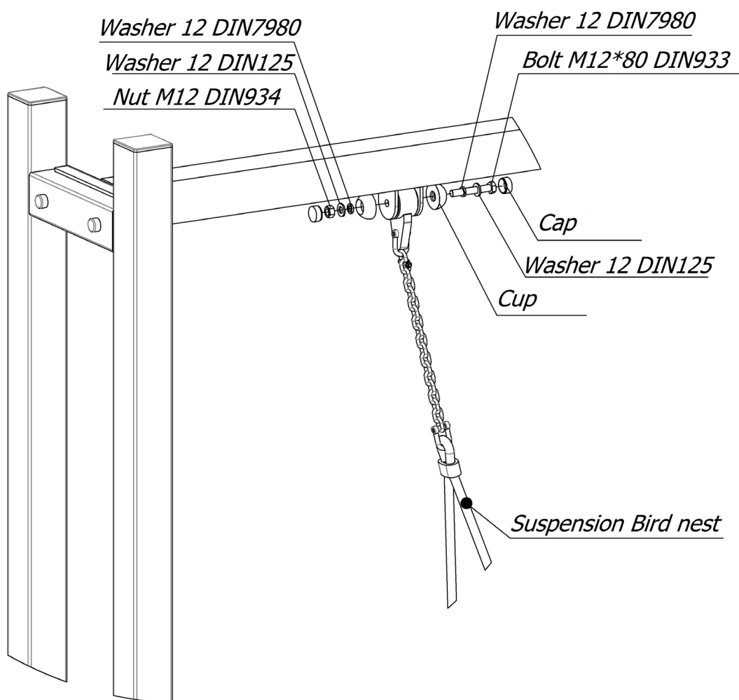
Picture 4 - Bird nest fastening scheme for the TE431-A
