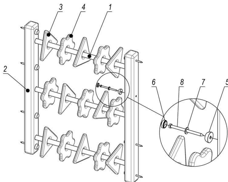
Picture 11 – Scheme of flag fastening
