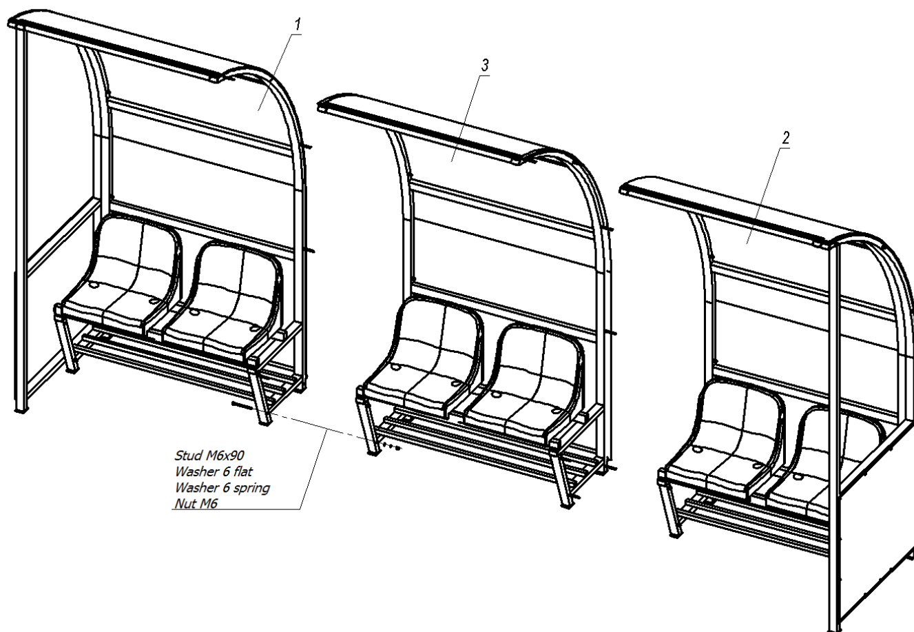
Picture 1 – Separating the product into its component parts
