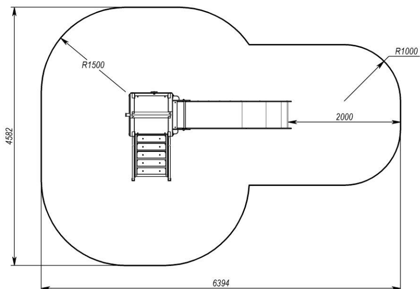
Picture 1 - Installation area and landing zone
