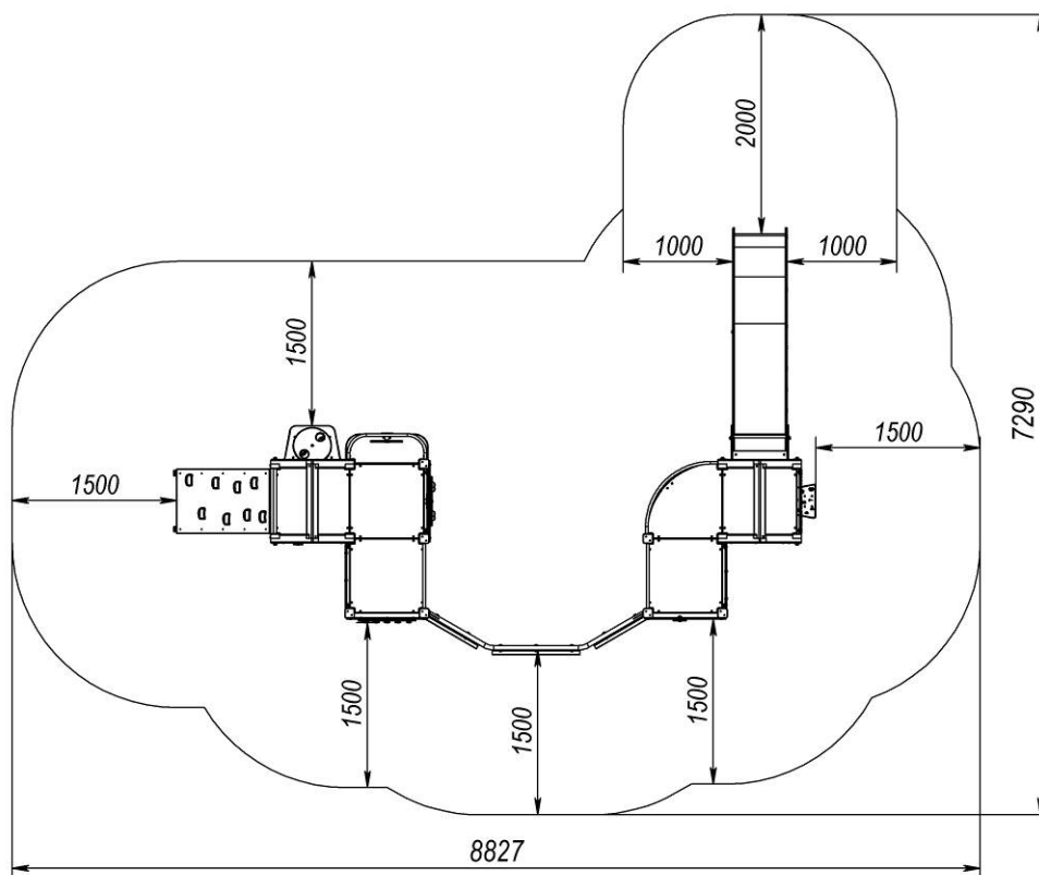
Picture 1 - Installation area and landing zone
