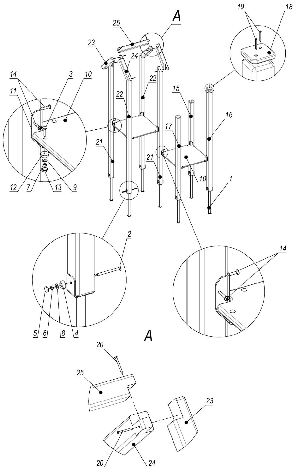
Picture 3 – Tower assembly scheme 1.23-0.75 m
