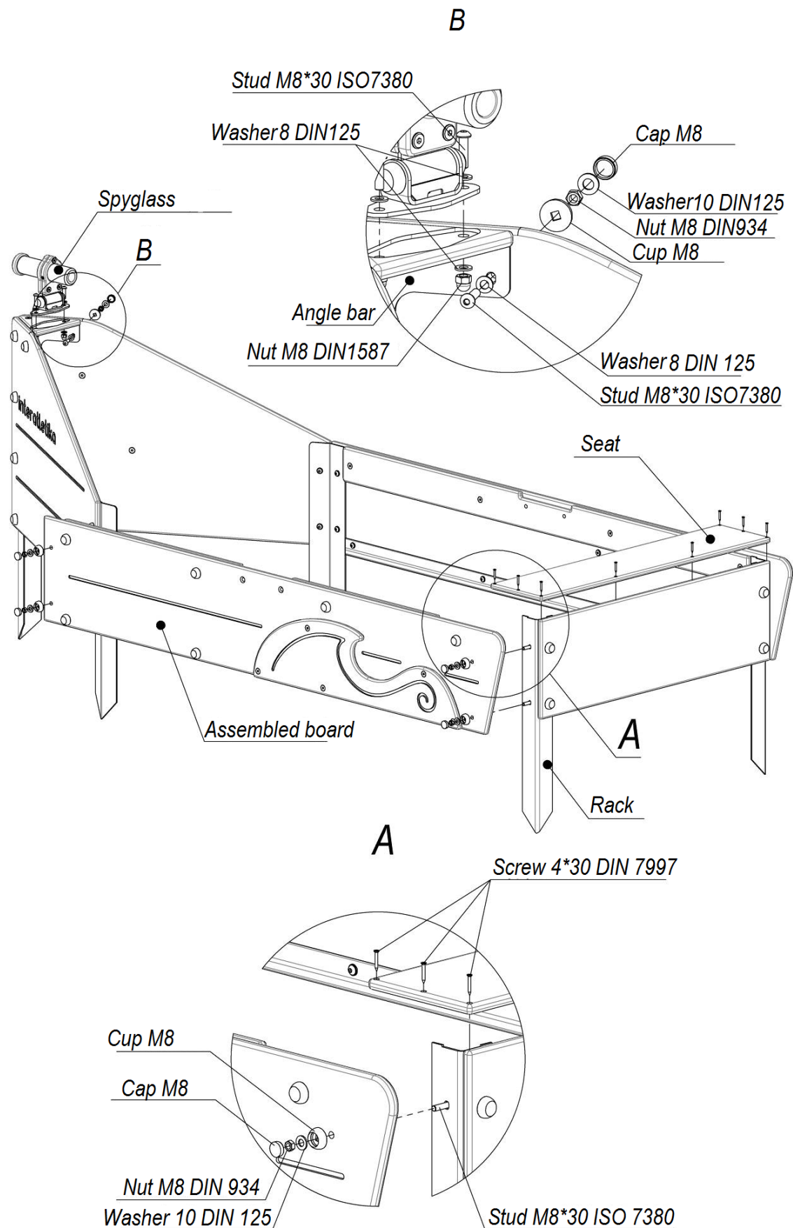
Picture 1 – Boards assembly scheme
