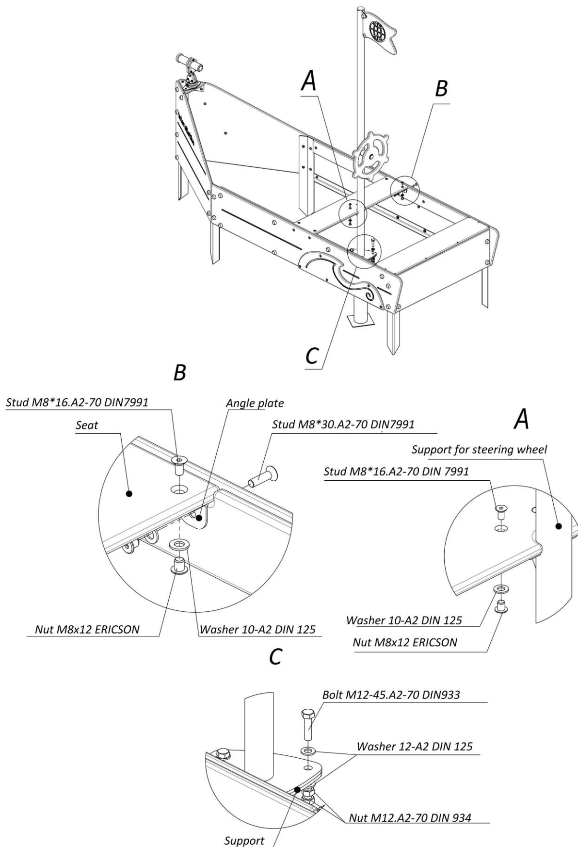
Picture 5 –Installtion scheme for steering wheel support with seat
