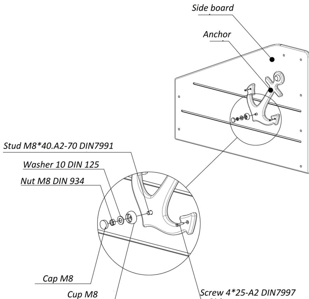
Picture 2 – Side board with anchor installation scheme
