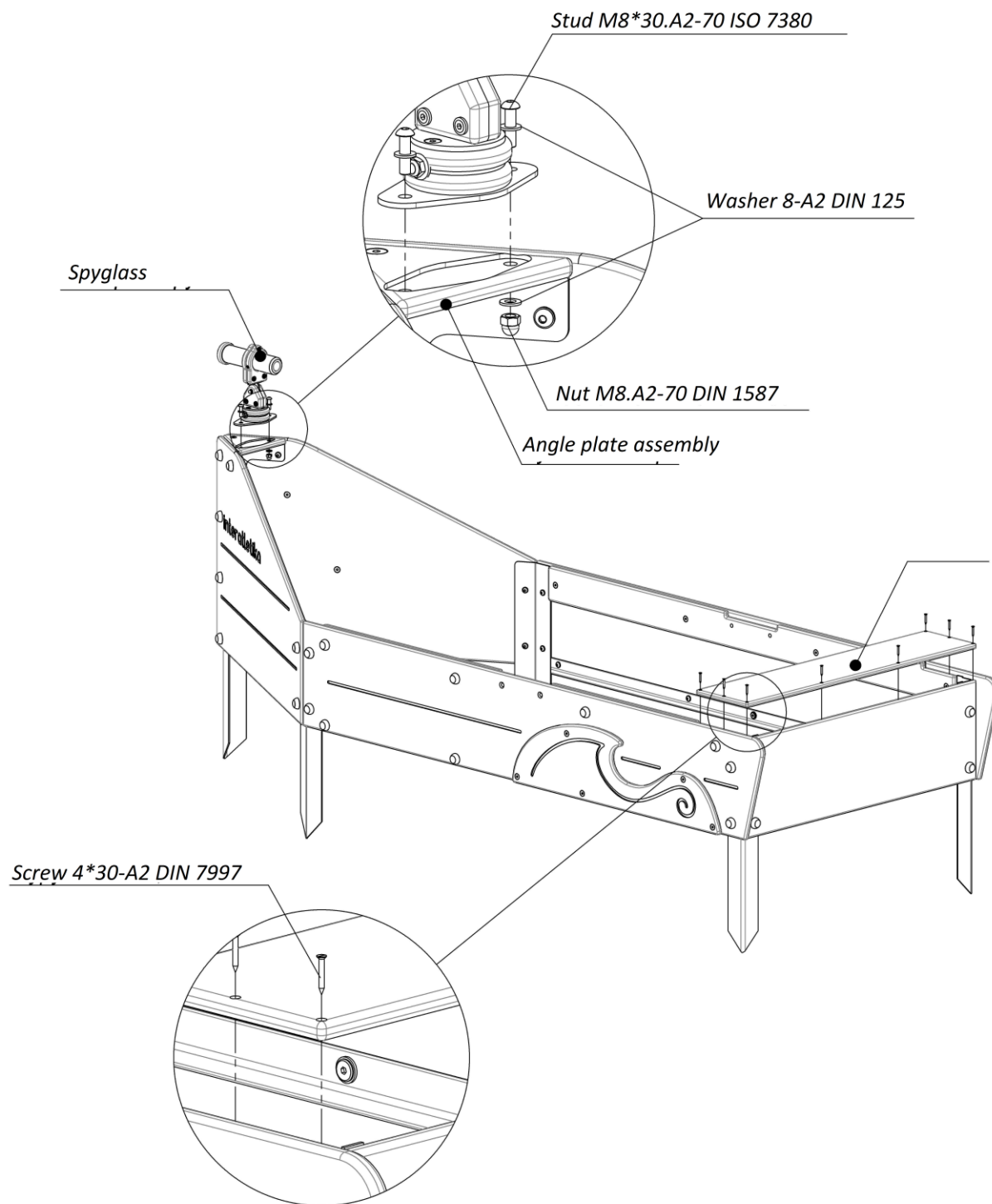
Picture 4 – Spyglass and seat installation scheme
