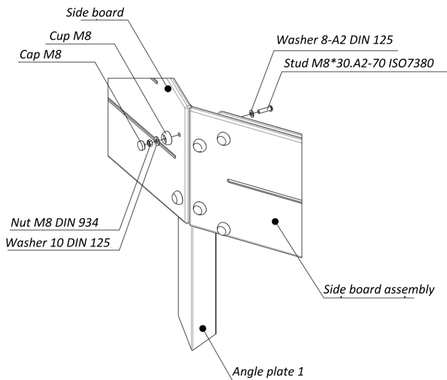
Picture 3 – Side board installation scheme. (Other elements of the sandbox installation scheme is identical)
