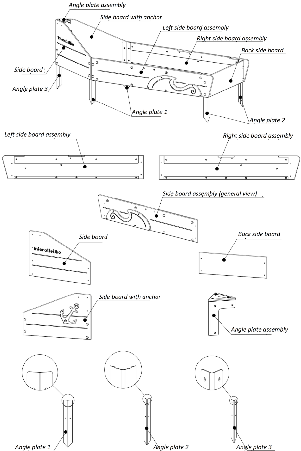
Picture 1 – Sandbox framework installation scheme
