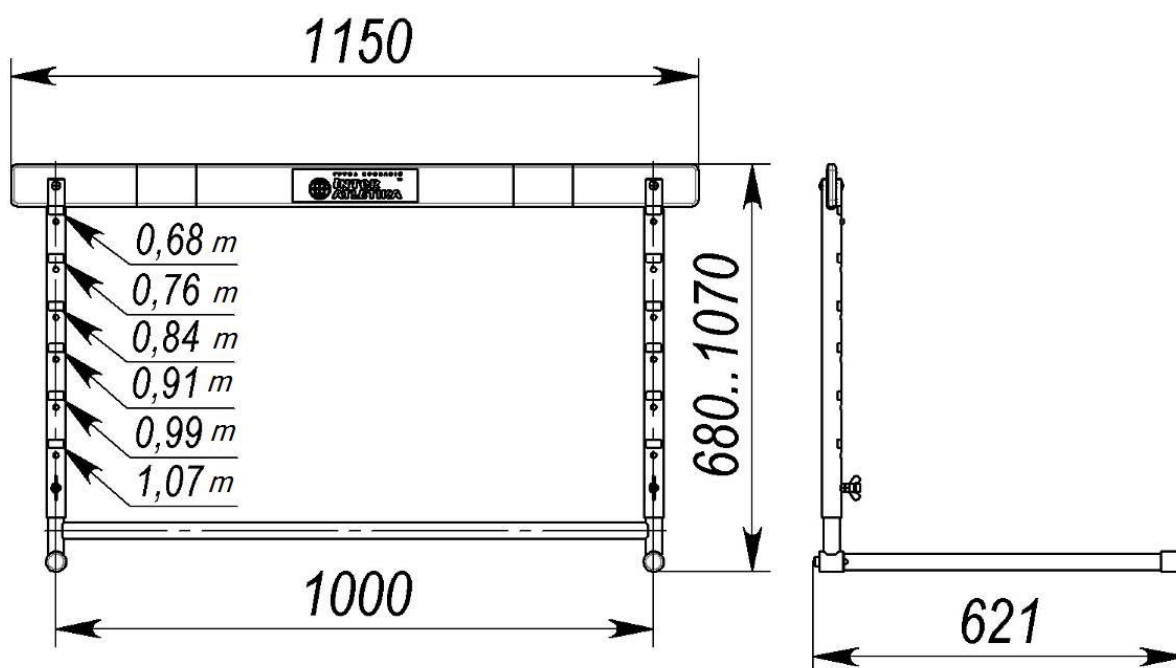
Picture 2 «Product overall dimensions and installation scheme»
