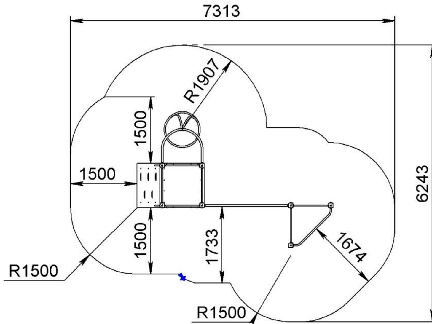
Pic.10 – Safety zone
