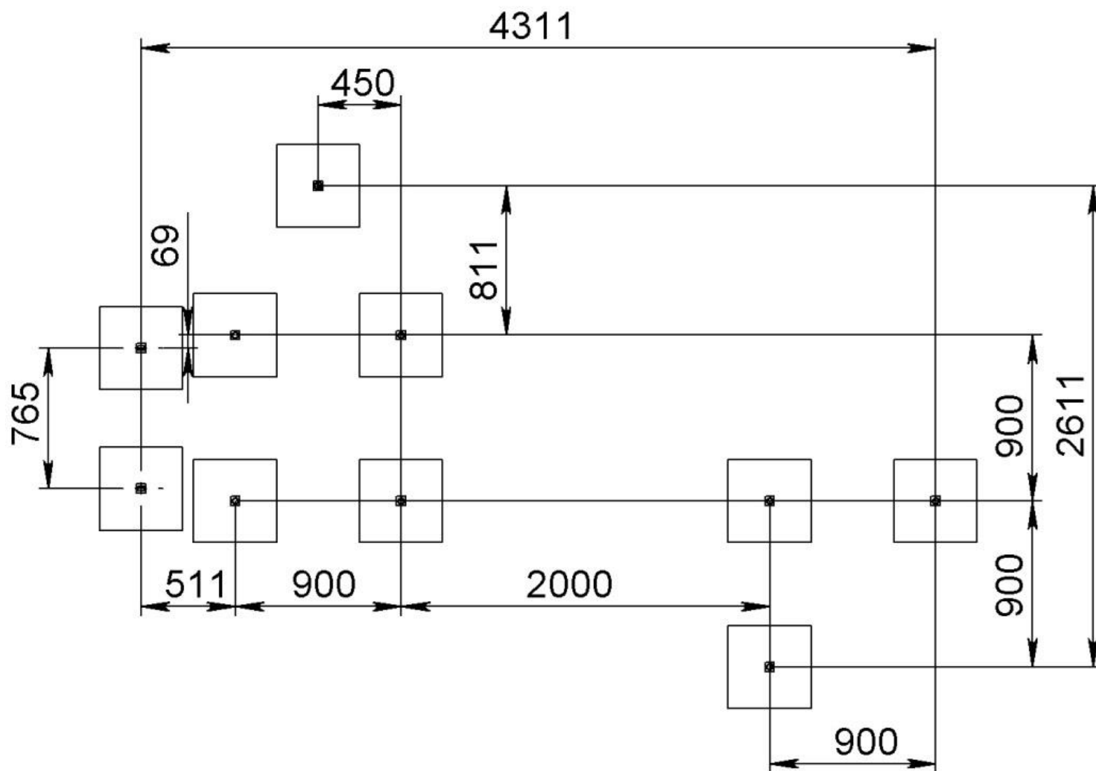
Pic. 11 – Layout of foundations
