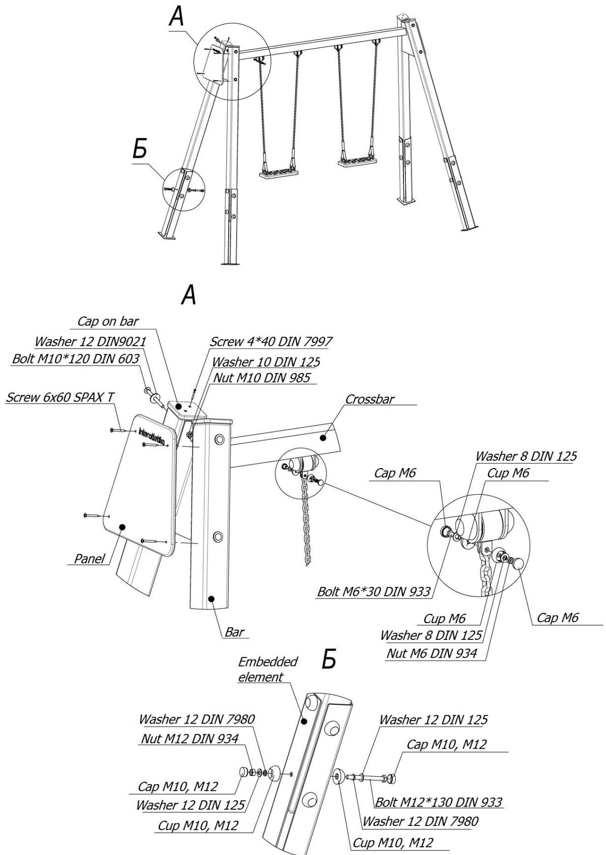
Picture 1 – Swing assembly scheme
