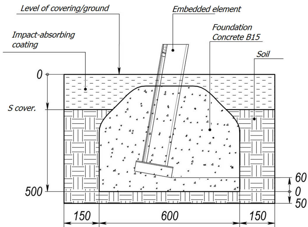
Picture 3 – Concreting scheme
