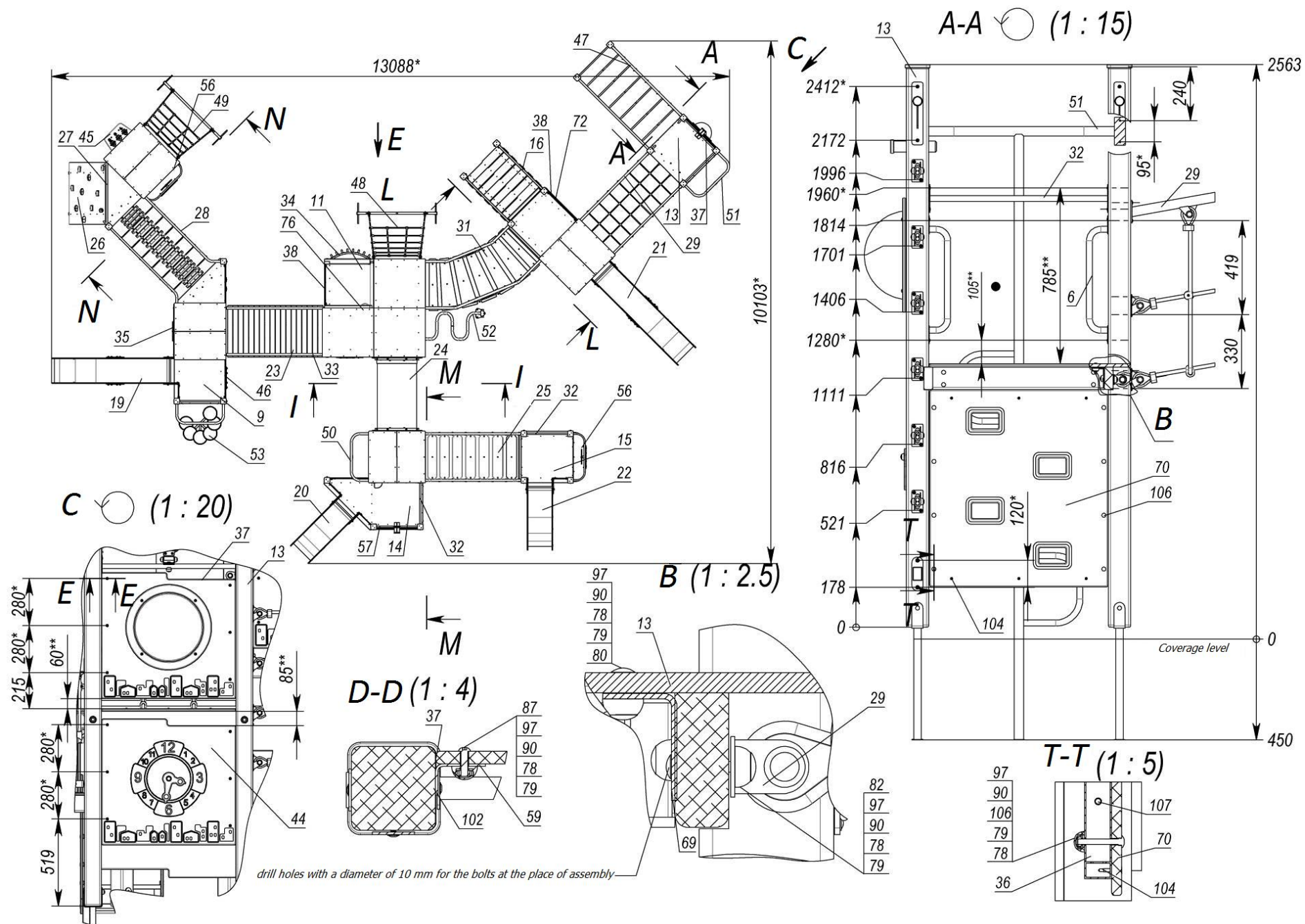
Picture 21 – Overall dimensions of the complex
