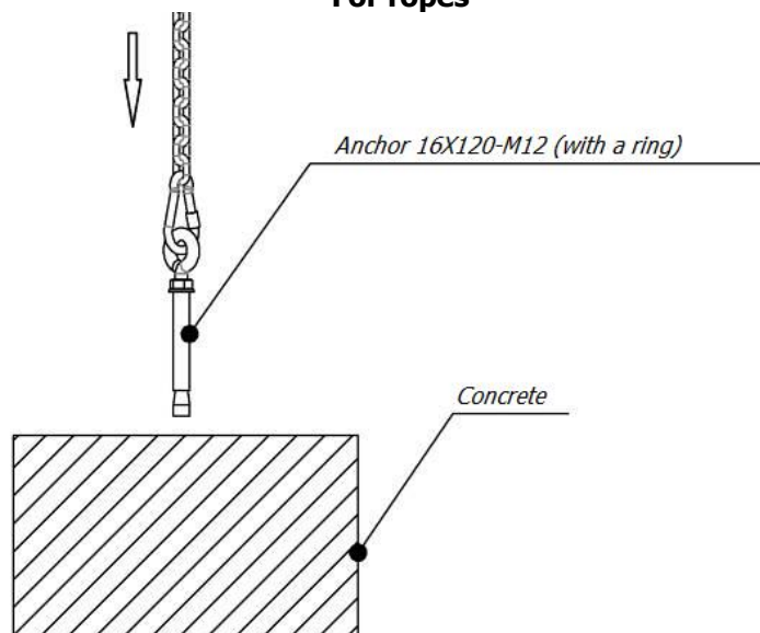
Picture 1.1 – Concreting scheme
