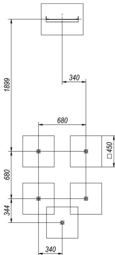
Picture 1 - Installation area and landing zone
