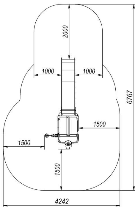
Picture 1 - Installation area and landing zone
