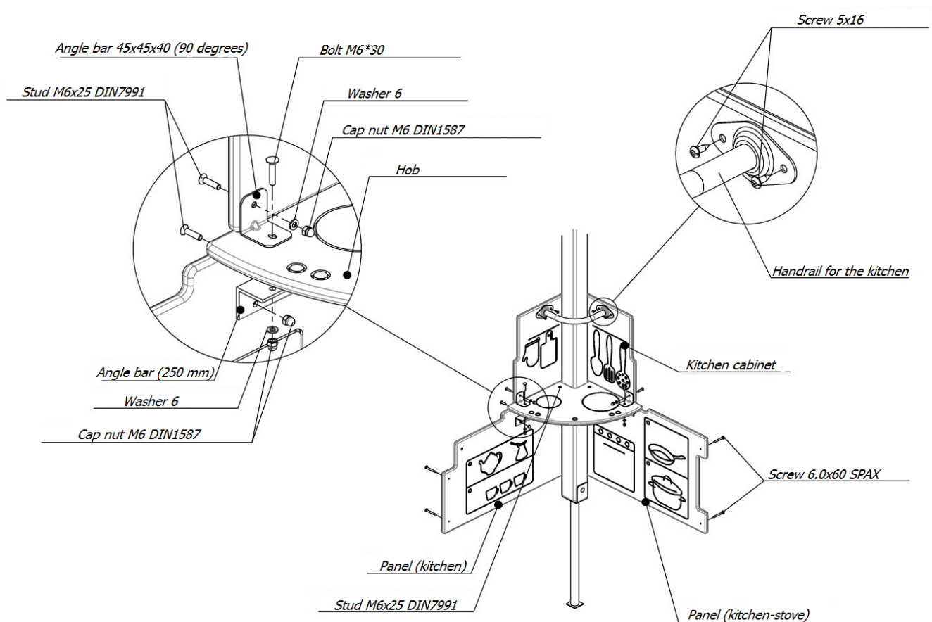
Picture 7 – Assembly scheme of the hob
