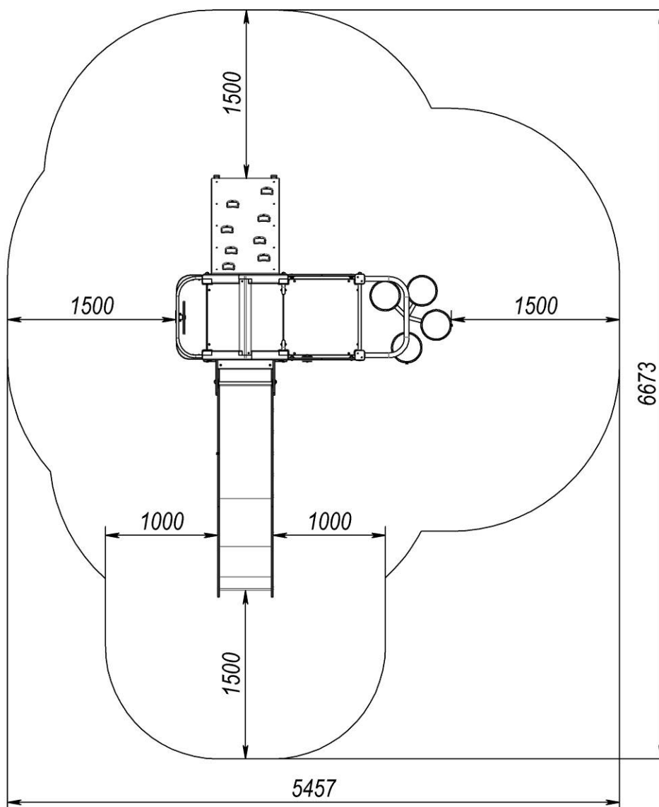
Picture 1 - Installation area and landing zone
