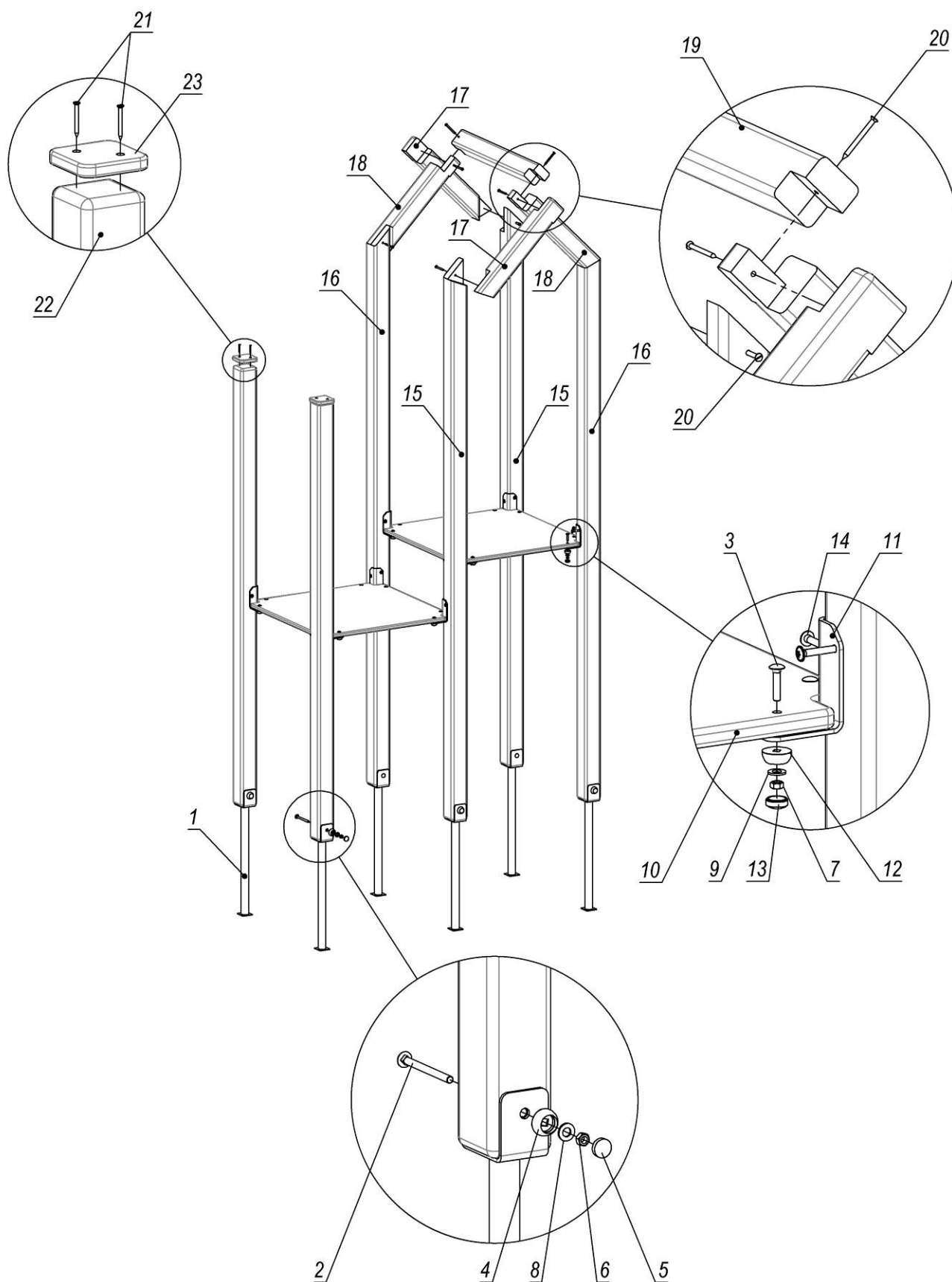
Picture 3 – Assembly scheme of double tower
