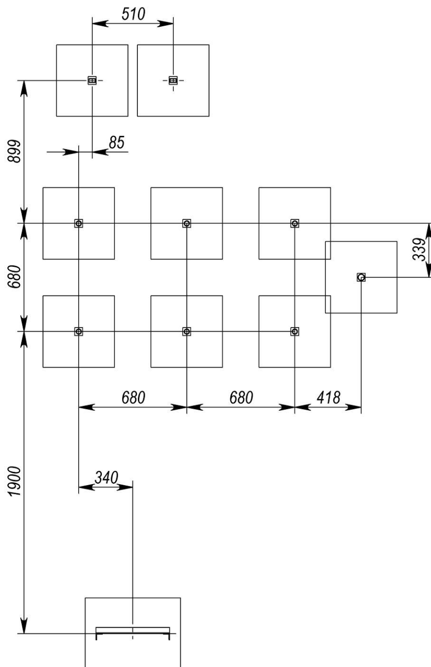
Picture 2 – Layout of the foundations
