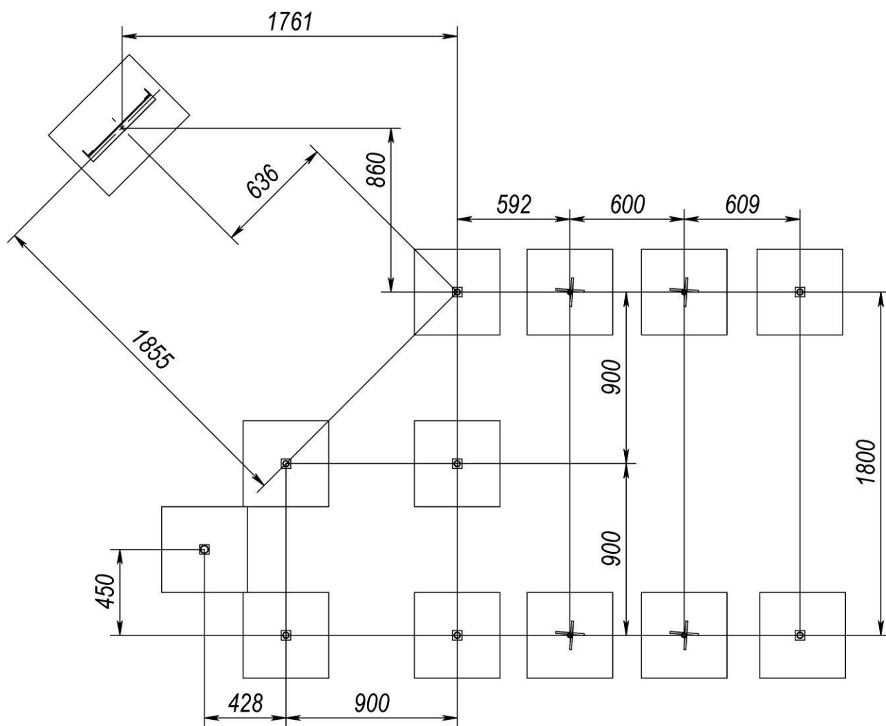
Picture 2 – Layout scheme of foundations
