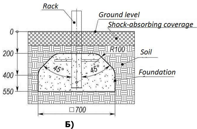
Picture 1 – Concreting scheme
