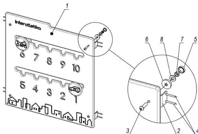
Picture 6 – Assembly scheme of stump
