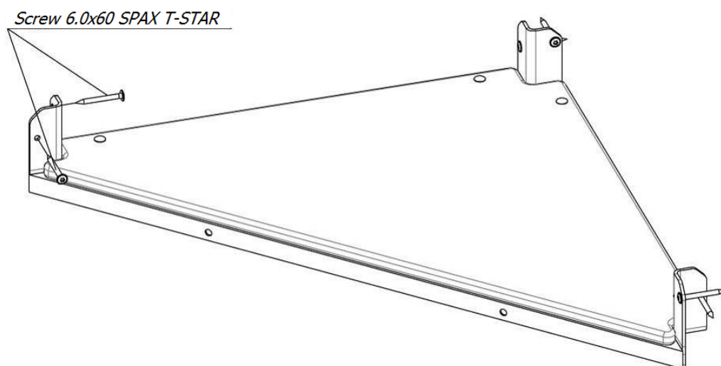
Picture 4 – Platform assembly scheme
