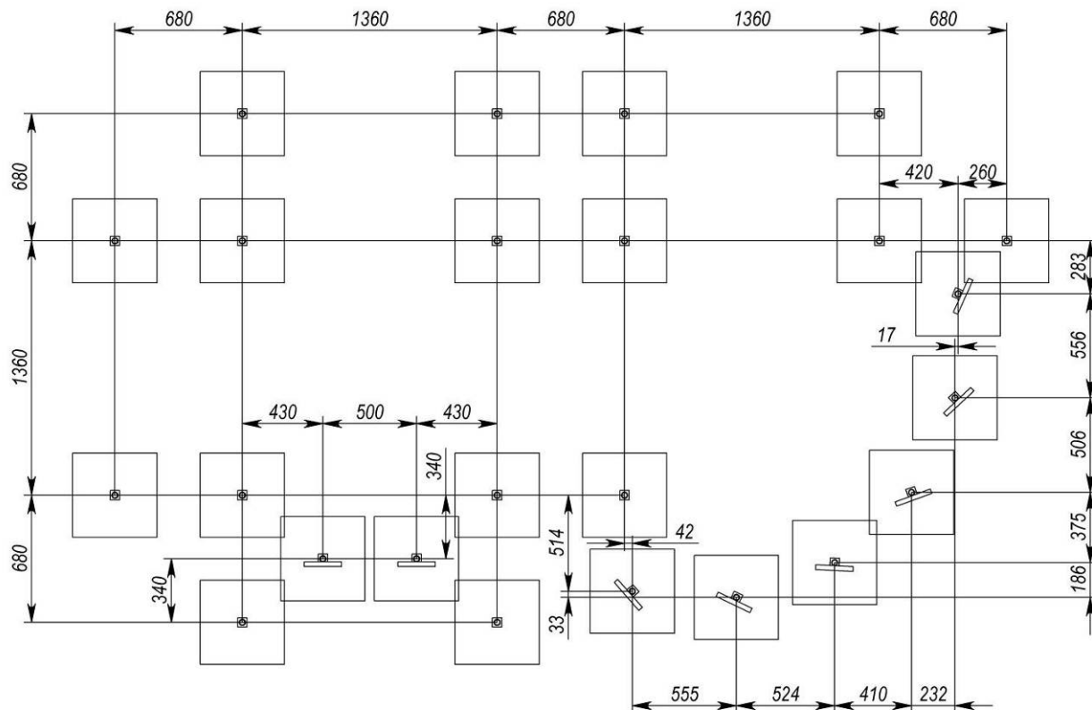
Picture 2 – Scheme of foundation layout
