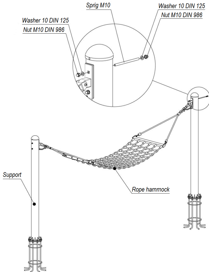
Picture 1 – «Rope hammock» installation scheme
