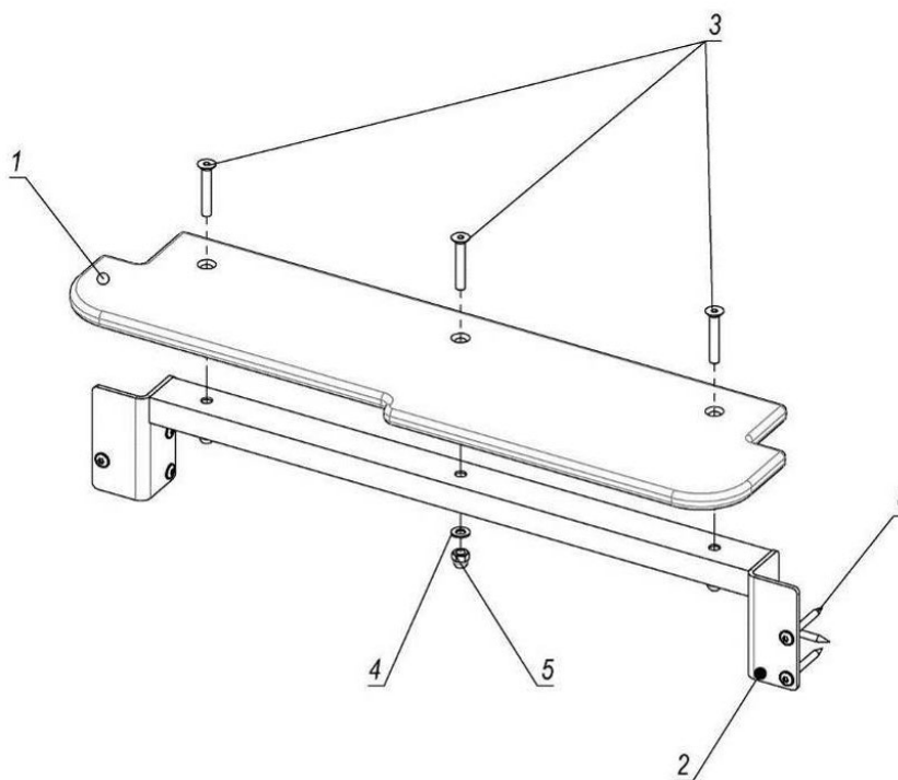
Picture 7 – Assembly scheme of the panel (assembly of other panels is identical)
