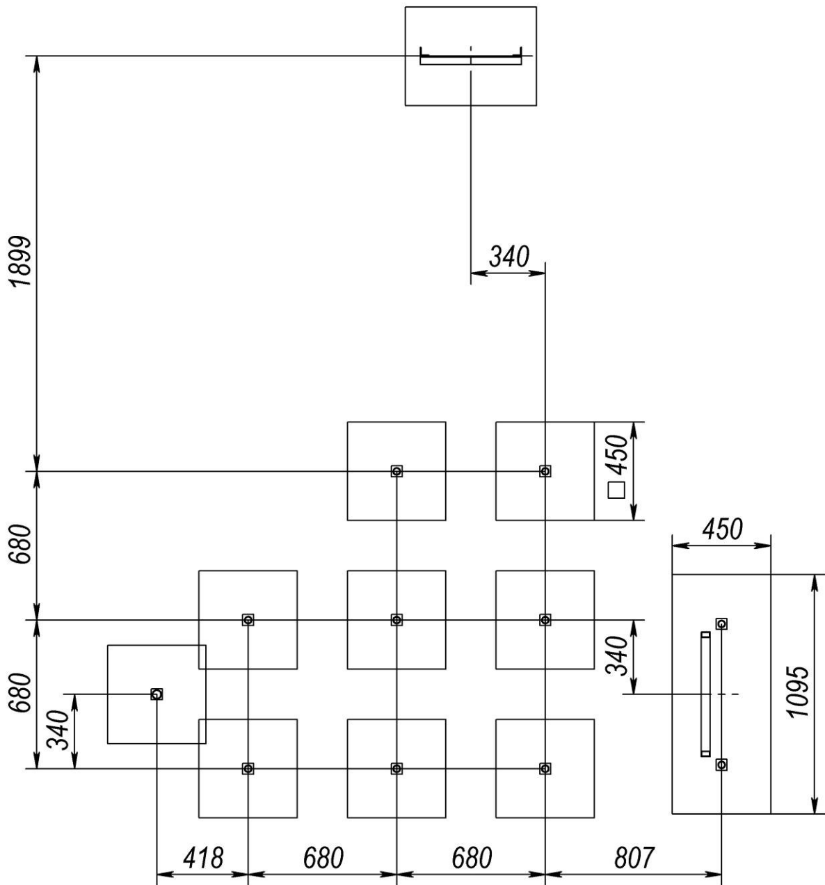
Picture 2 – Layout of the foundations
