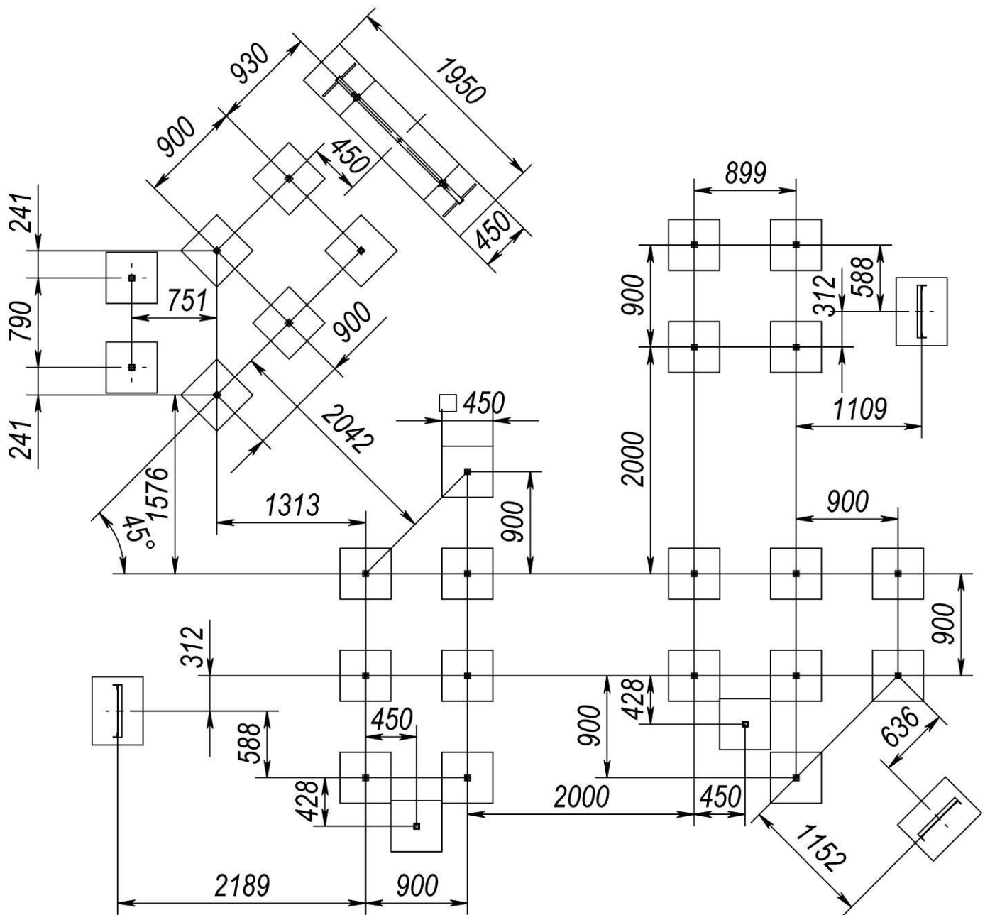
Picture 2 – Layout of foundations
