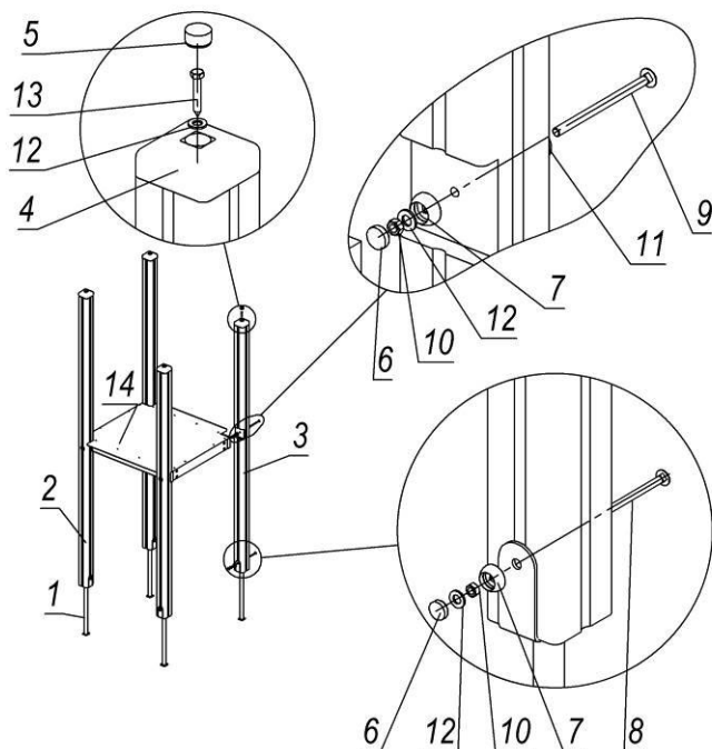
Picture 8 – Components and assembly scheme of the 1.5 m tower with caps (1.5 m - height of the platform from ground level)
