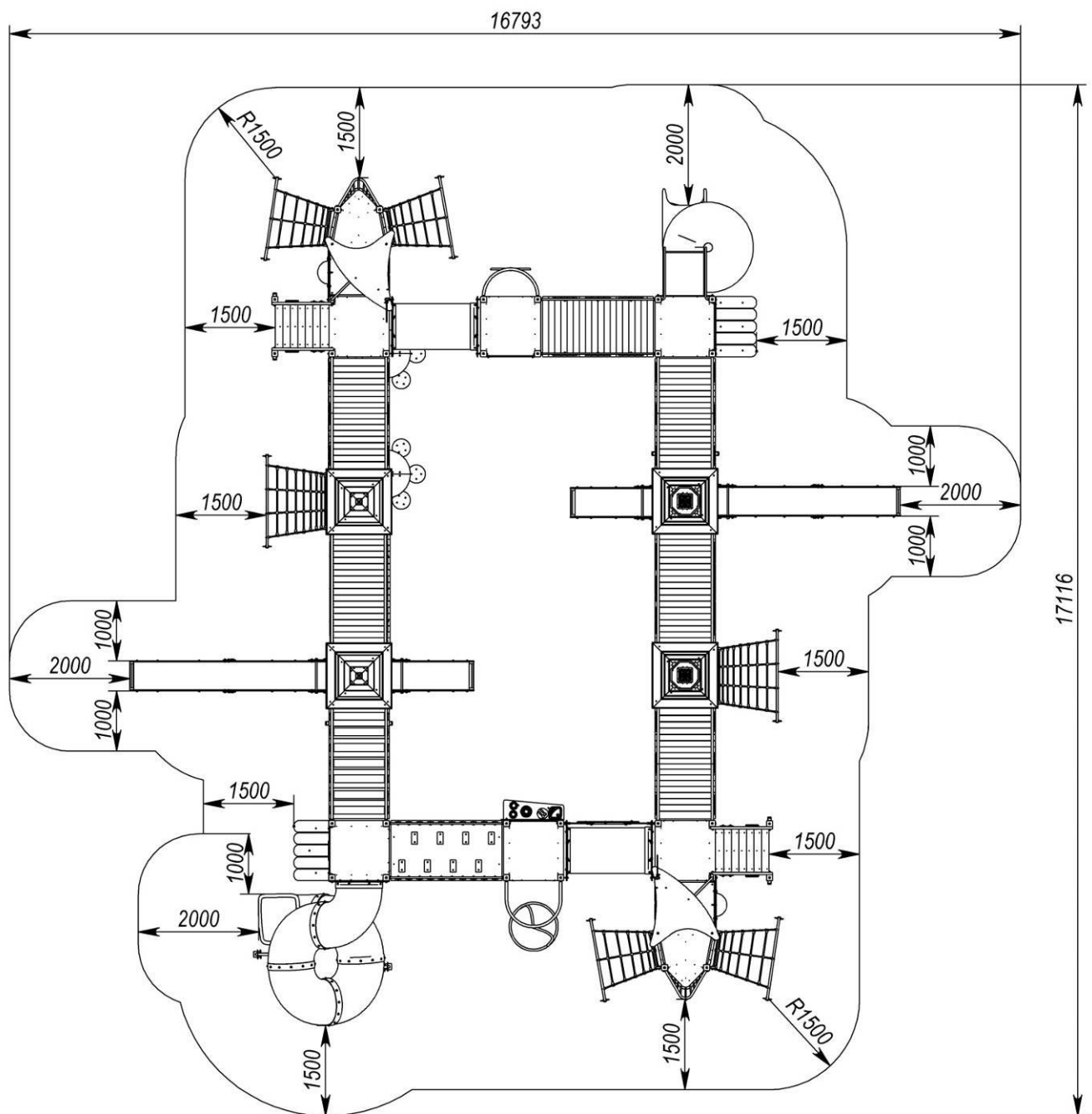
Picture 38 - Layout of the safety zone
