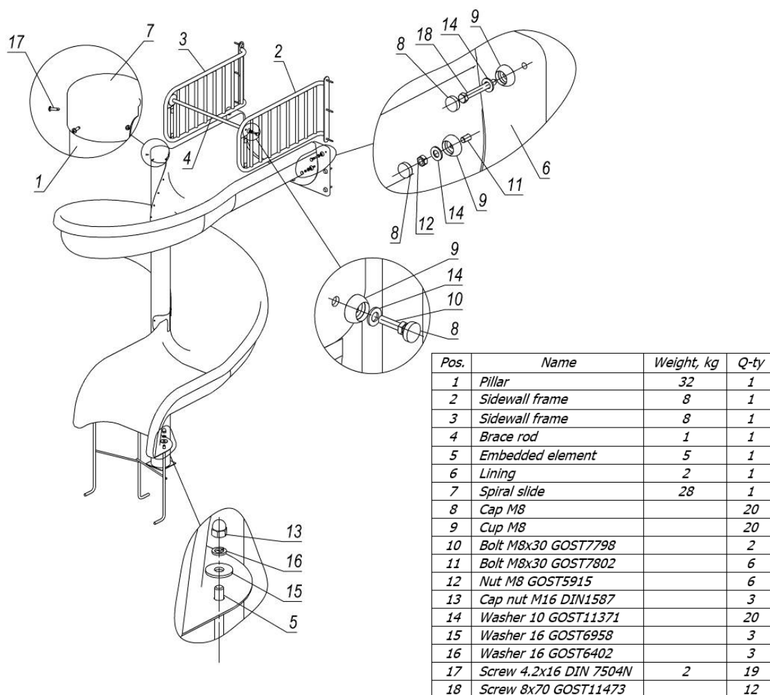
Picture 16 - Install a 2 m slide to the tower with two platforms 0.7-2 m from the ground:
