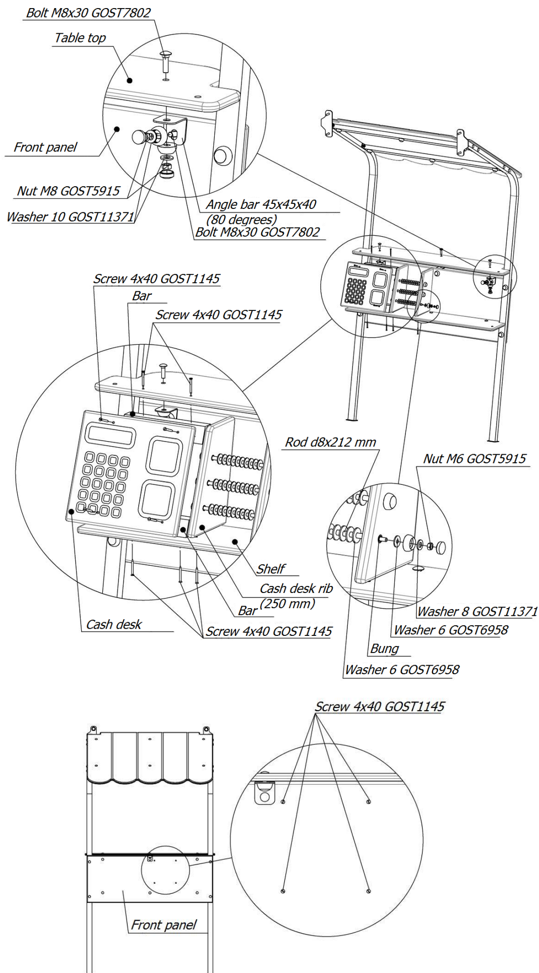
Picture 30 – Fixing scheme of the canopy
