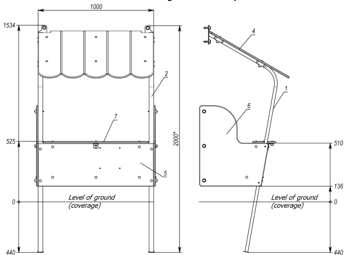
Picture 32 – Fixing scheme of the panel
