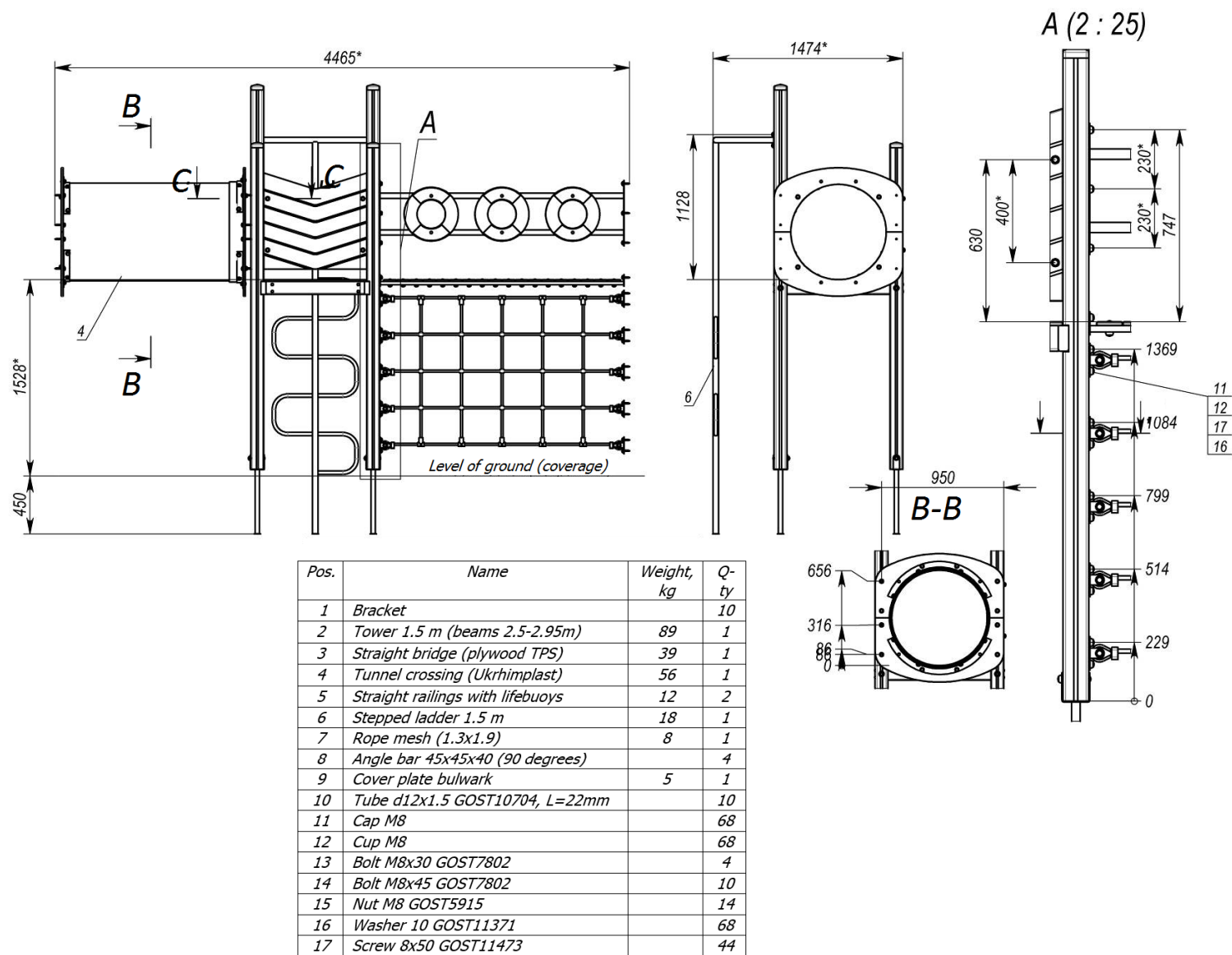
Picture 6 - Completeness and main characteristics of the third part
