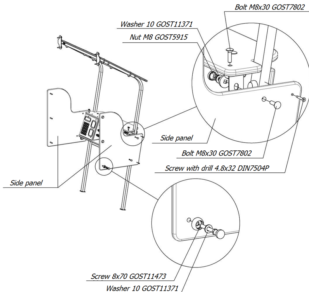
Picture 31 – Assembly scheme of the cash desk
