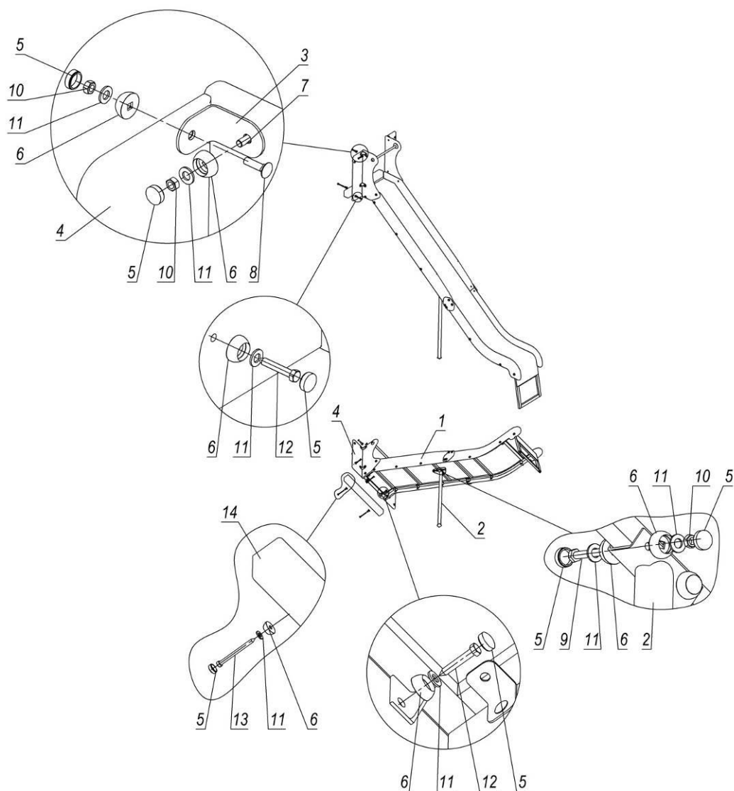
Picture 17 - Place a spiral descent to one of the towers (platform height -1.5 m)
