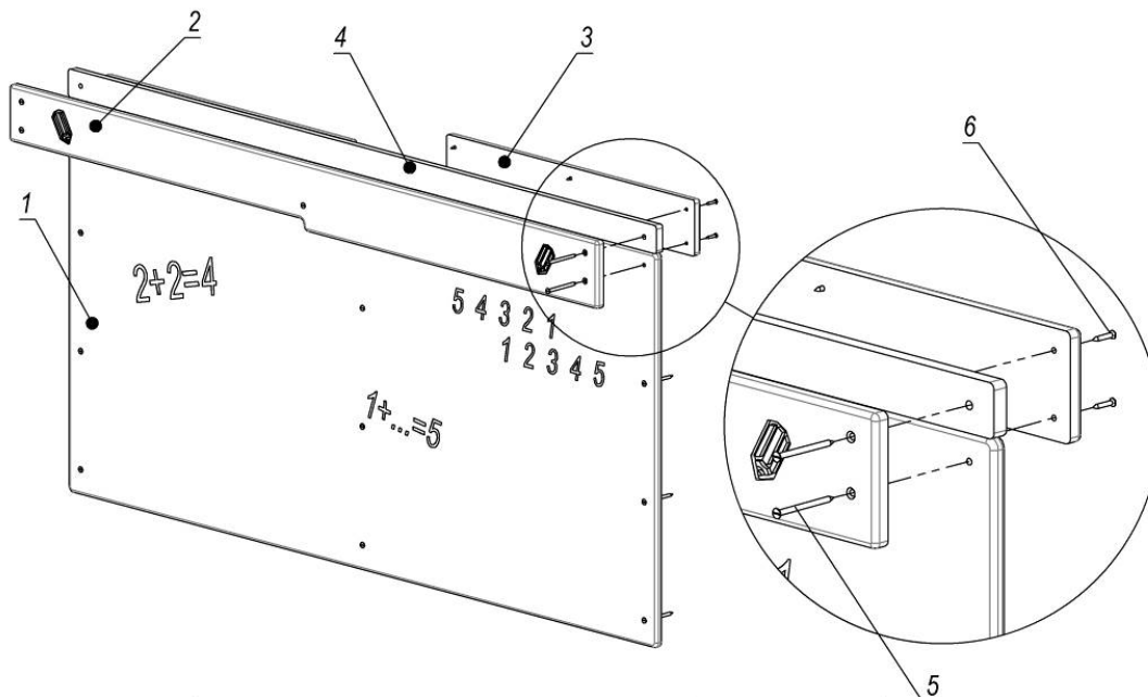
Picture 9 – Assembly scheme of the intercom
