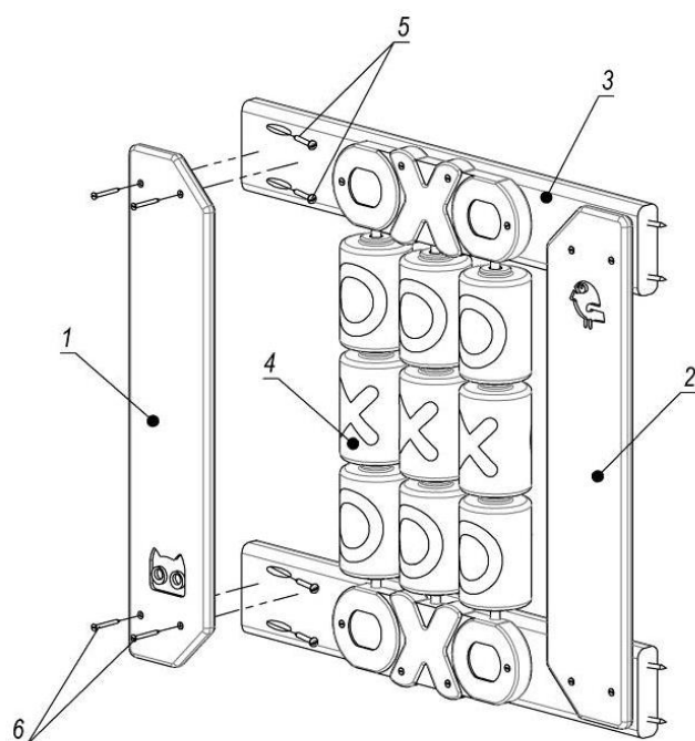
Picture 7 – Assembly scheme of the counting frame
