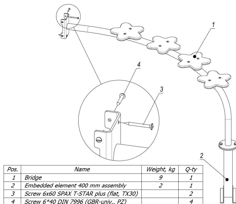
Picture 4 – Scheme of fastening the 'Bridge'
