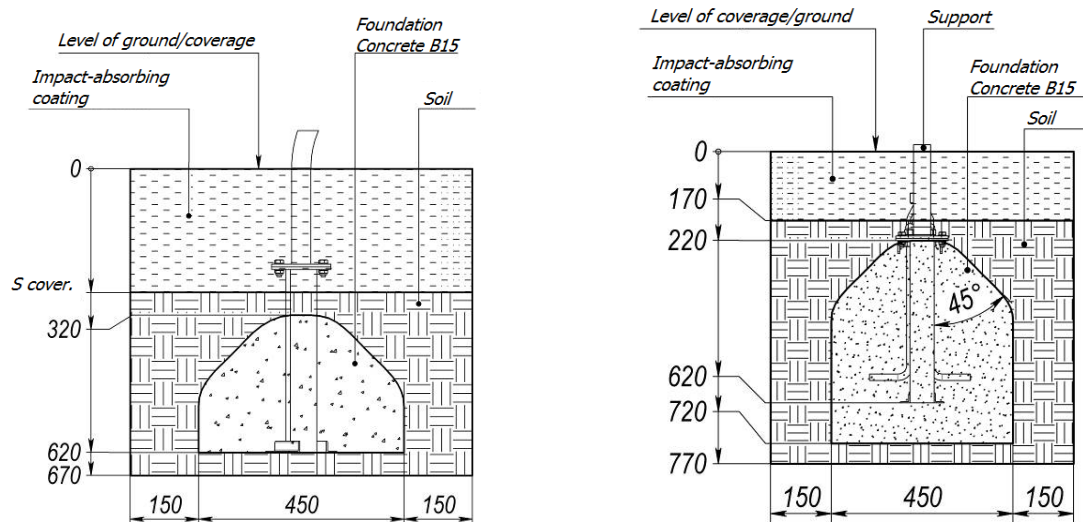
Picture 5 – Concreting schemes
