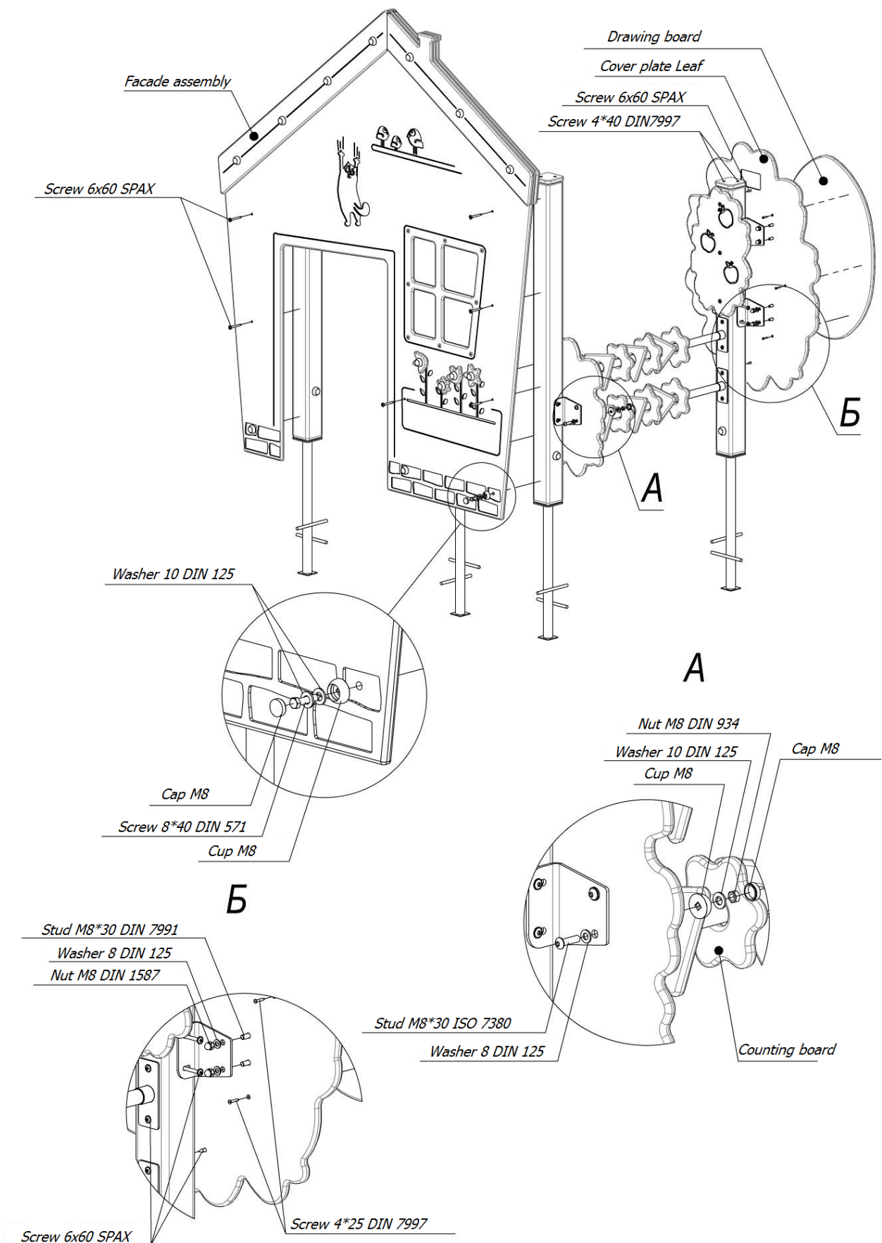
Picture 2 – Installation scheme of the 'Facade, counting, drawing board'
