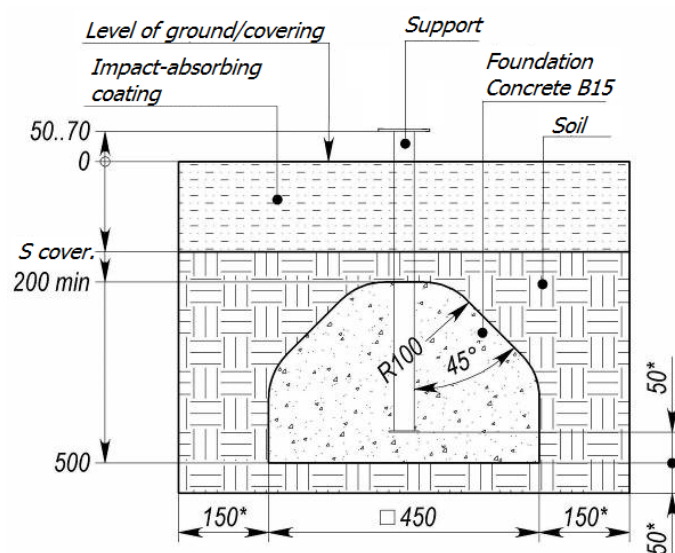
Picture 4 – Scheme of fastening the 'Bridge'
