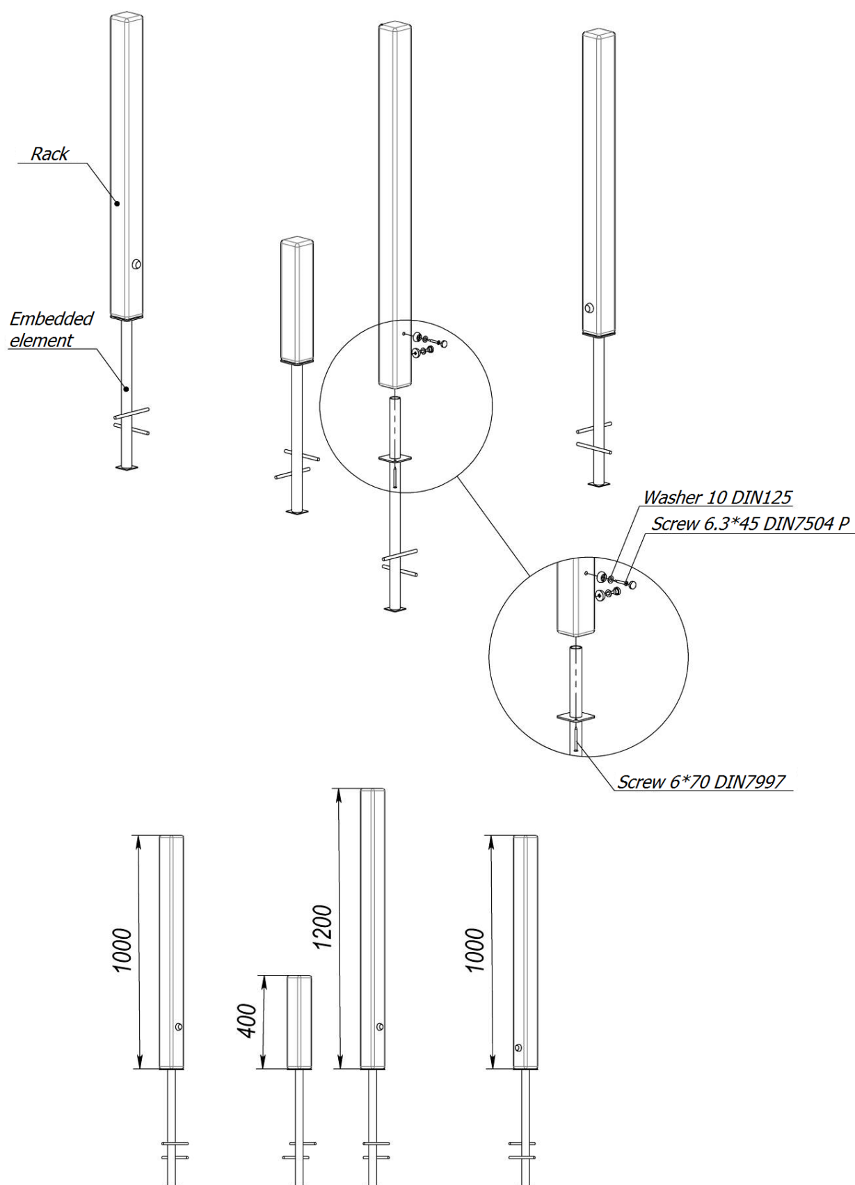
Picture 1 – Installation scheme of the racks
