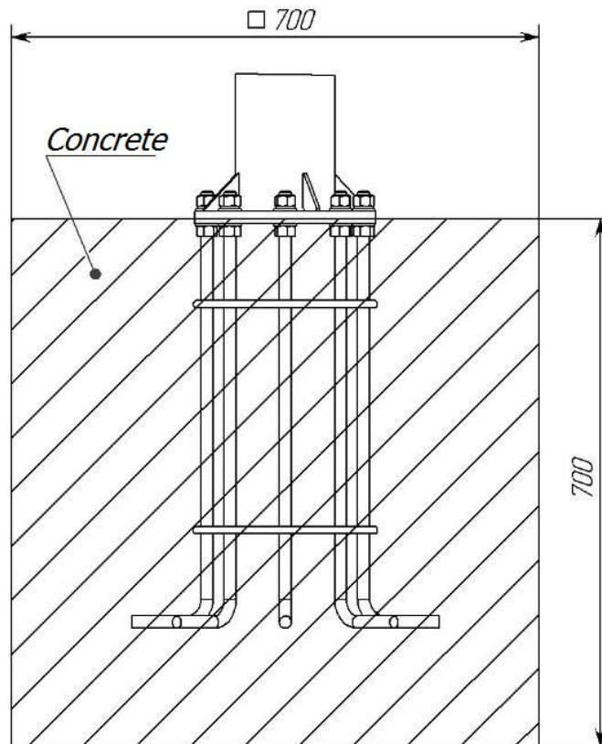
Picture 5 – Concreting scheme
