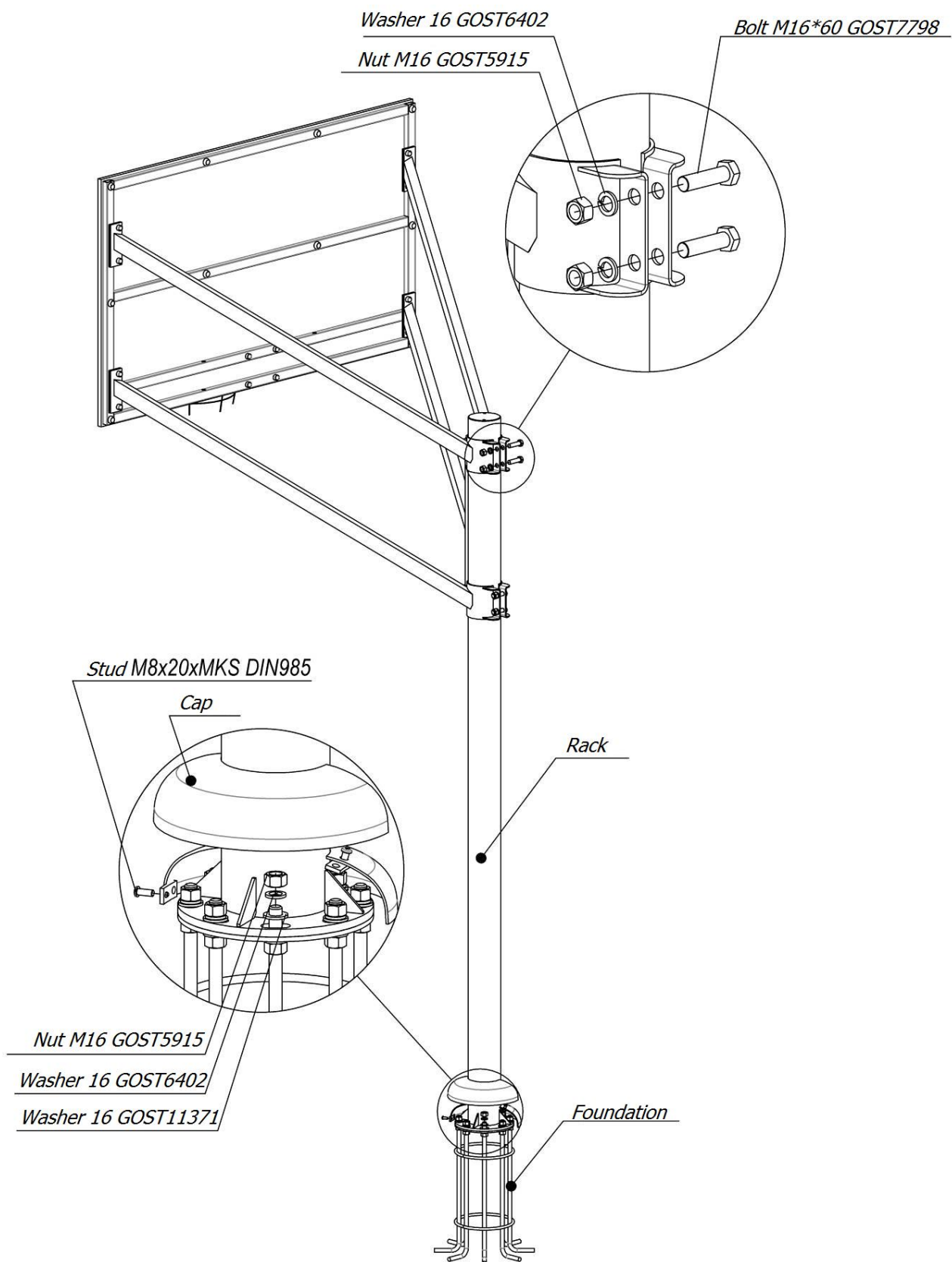
Picture 4 – Installation scheme 2
