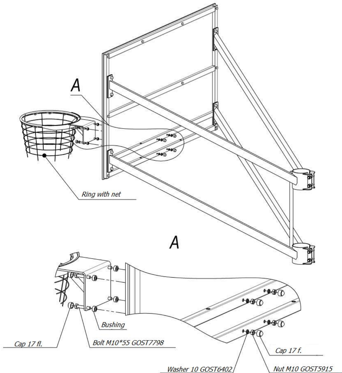
Picture 3 – Installation scheme of Ring with net for UT417.1
