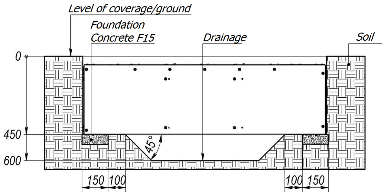
Picture 1 – Installation scheme
