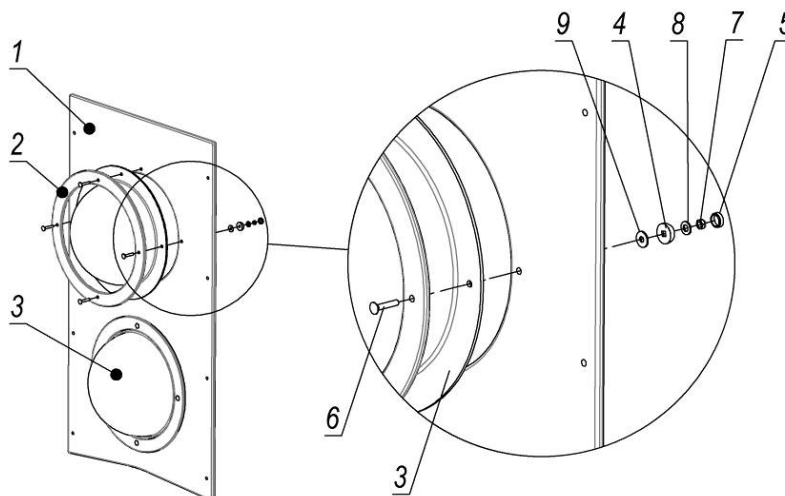
Picture 20 – Completeness and assembly scheme of «Panel workshop»
