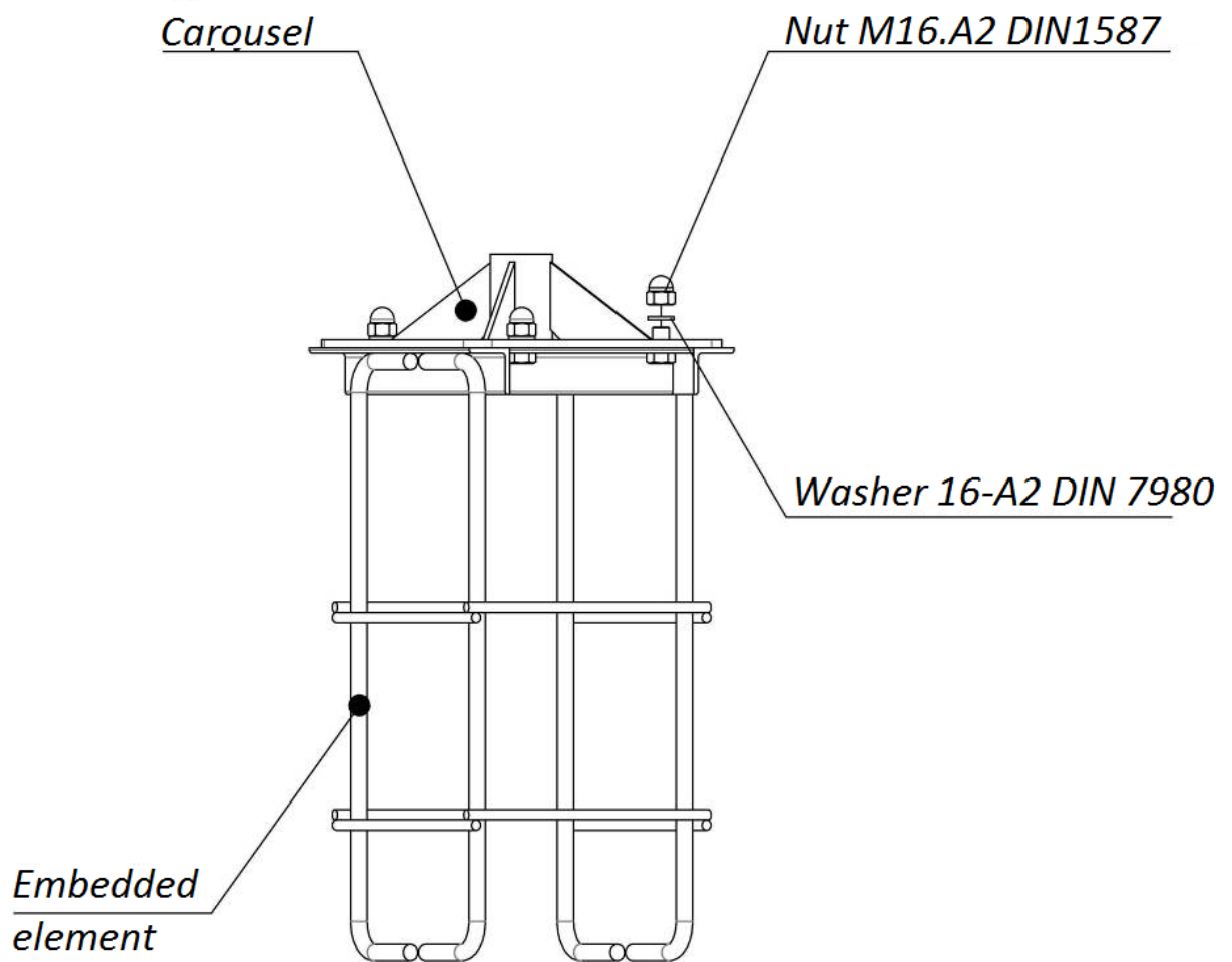
Picture 3 – Carousel and embedded element connection scheme
