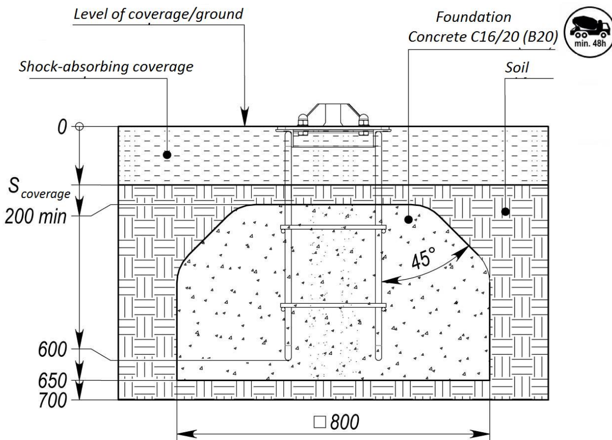
Picture 5 – Concreting scheme
