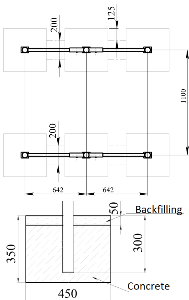
Pic. 3 Scheme of foundation installation
