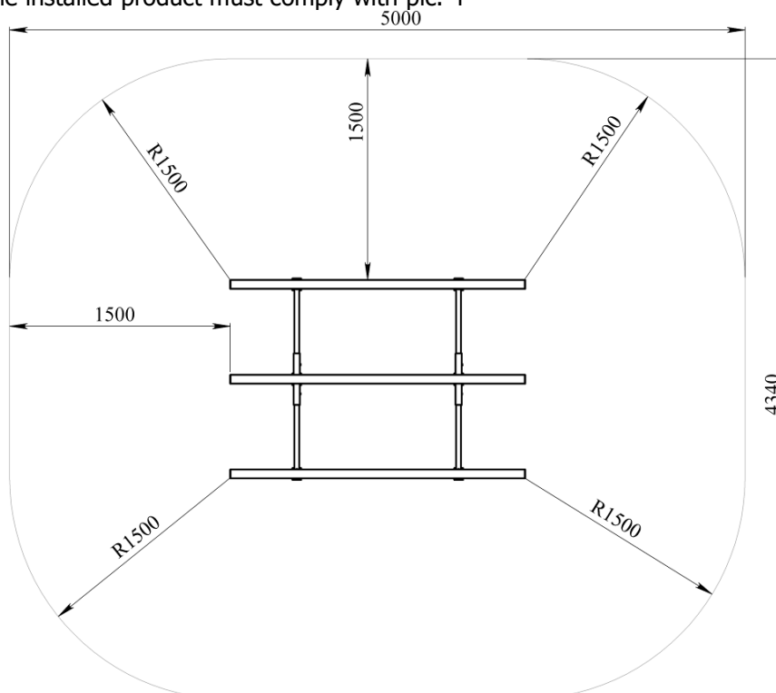
Pic. 4 Safety zone
