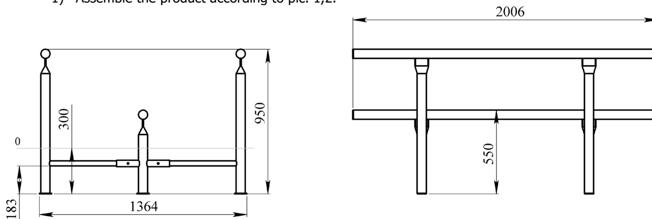
Pic. 2 Overall dimensions
