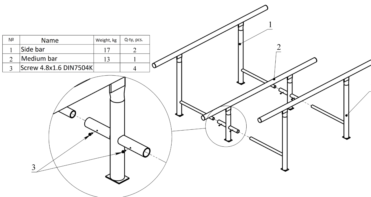
Pic. 1 Components and assembly procedure
